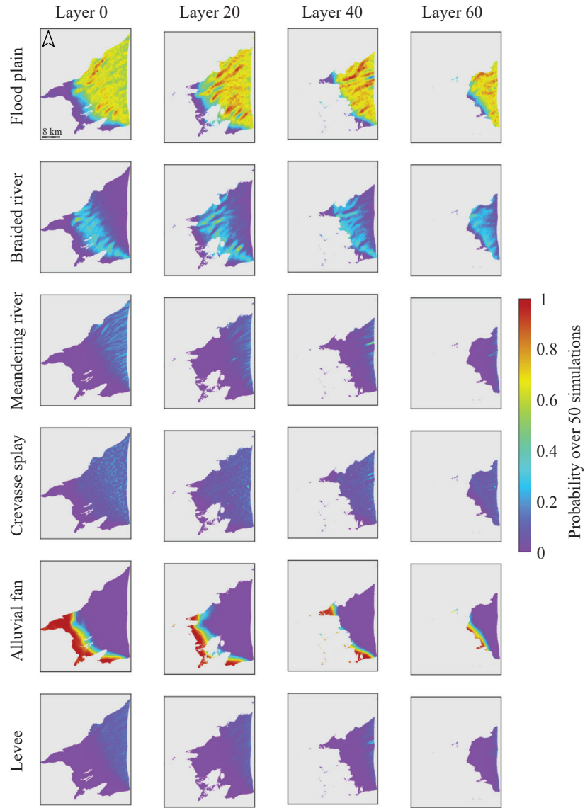
Figure 8. Probability maps of the six simulated facies at different depth. The probability maps are calculated over a 50 simulations set.
