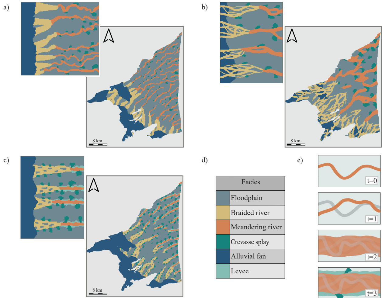
Figure 2. Horizontal training images (TIs) associated with their corresponding 2D MPS simulations. a) analog TI derived from satellite images of the Tagliamento river, b) a conceptual analogue TI and c) a TI created based on outcrop descriptions and general knowledge of the Roussillon's plain. d) the six sedimentary facies of the final TI. e) illustration of the sedimentological concept for the creation of the final TI, the aim is to simulate the area of high river bed occurrences (channel belt) rather than individual river channels.
