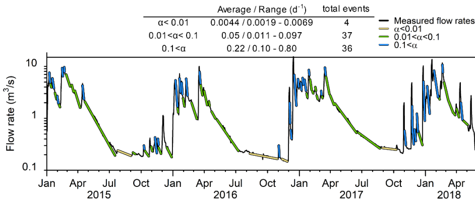
630 Figure 6: Calibration of the recession coefficients for 77 depletions over the 2015-2018 period.
