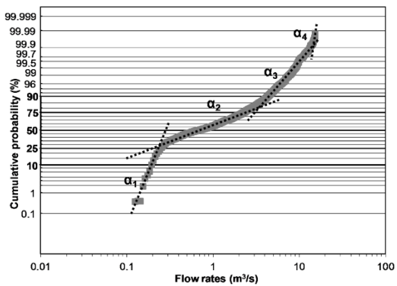
625 Figure 4: Cumulative probability of flow rates and their classification by slope ( \alpha_1 to \alpha_4 ) for the 2015-2018 period.
