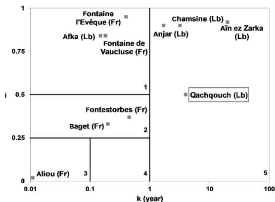
610 Figure 5: Qachqouch spring within the classification of karstic springs as a function of their k and i parameters (El-Hakim and Bakalowicz, 2007). Fr = France and Lb = Lebanon.
