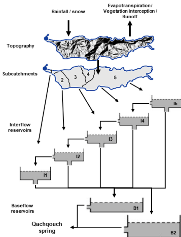
Figure 3: Conceptual map of the model, using the internal structure of MIKE SHE (DHI, 2016a, 2016b).
