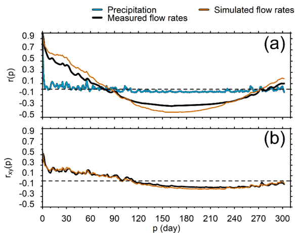
615 Figure 7: Autocorrelation functions of precipitation, measured flow rates, and simulated flow rates (a) and cross-correlation functions between precipitation (input) and measured or simulated flow rates (outputs) (b). Both were performed on 1/3 of the 2015-2018 period ( m = n/3 ).
