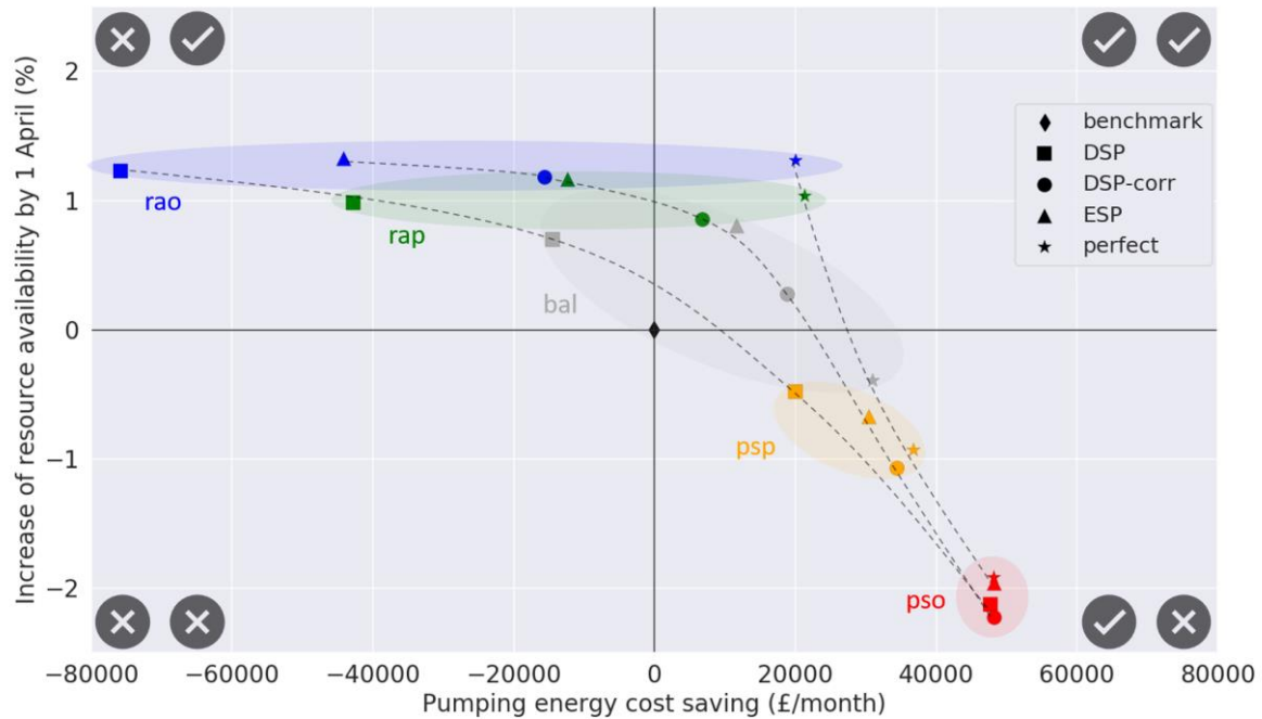
680 Figure 4 Post-evaluation Pareto fronts representing the average system performance improvement (over period 2005-2016) of the 685 real-time optimization system during the pumping licence window (1 Nov - 1 Apr) with respect to the benchmark (black diamond), using four forecast products: non-corrected forecast ensemble (DSP), bias corrected forecast ensemble (DSP-corr), ensemble streamflow prediction (ESP) and perfect forecast. For each of the four forecast products, five scenarios of operational priorities are represented: resource availability only (rao; in blue), resource availability prioritised (rap; in green), balanced (bal; in grey), pumping savings prioritised (psp; in green) and pumping savings only (pso; in red). For visualization purposes, the coloured circles group points under the same operational priority scenario and the dashed lines link points using the same forecast product. The pumping energy cost is calculated as the sum of the energy costs associated to pumped inflows and pumped releases and the resource availability as the mean storage volume in both reservoirs (S1 and S2) at the end of the optimisation period. Both objective values are rescaled with respect to the performances of the benchmark operation.
