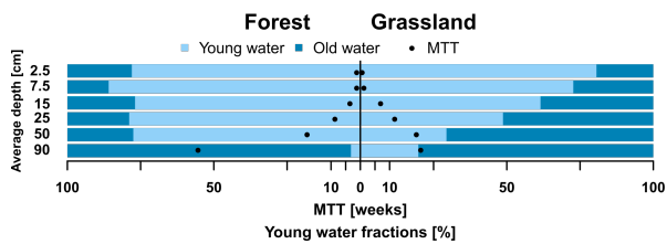
Figure 6. Young water fractions and MTT per soil depths at forested and grassland site.
