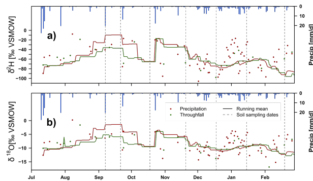
Figure 4. Time series of daily precipitation amount and isotopic signature of weekly and daily precipitation and their 30 days running (volume weighted) mean for \delta^2\text{H} (a) and \delta^{18}\text{O} (b) with dotted lines indicating dates of bulk soil water sampling (- -).
