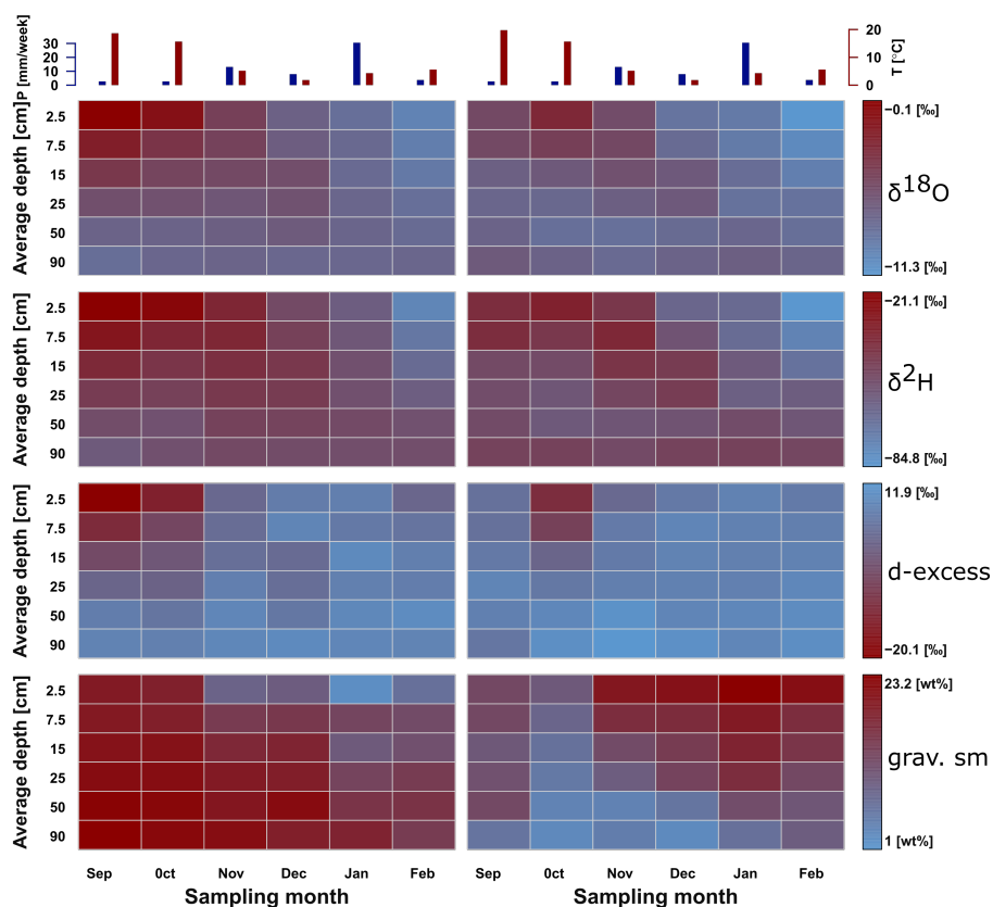
Figure 5. Heat map of soil depth profiles for mean \delta^2\text{H} , \delta^{18}\text{O} , d-excess and grav. soil moisture of three replicates at both land use classes (forest & grassland) of six monthly sampling dates. Blue to red colours indicate more to less depleted \delta^2\text{H} & \delta^{18}\text{O} values, declining d-excess, and grav. soil moisture values. On top, antecedent conditions of mean daily air temperature and sum of precipitation 7 days prior to sampling are displayed in the bar chart.
