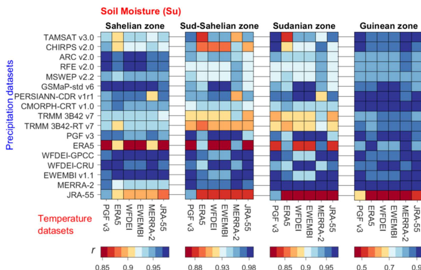
355 Figure 5. Pearson correlation coefficient ( r ) of modelled soil moisture ( S_u ) compared to ESA CCI data over the simulation period (2003-2012) considering 102 combinations of rainfall (y-axis) and temperature datasets (subplots on x-axis) used as forcing for the hydrological model.
