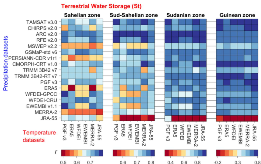
Figure 4. Pearson correlation coefficient ( r ) of modelled terrestrial water storage compared to GRACE data in four climatic zones in the Volta River basin over the simulation period (2003-2012) considering 102 combinations of rainfall (y-axis) and temperature datasets (subplots on x-axis) used as forcing for the hydrological model.
