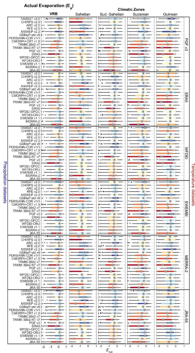
415 Figure 10. Spatial pattern efficiency ( E_{SP} ) of actual evaporation ( E_a ) over the entire simulation period (2003-2012) for the Volta River basin (VRB) and its climatic zones, using different combinations of precipitation and temperature datasets used as input for hydrological modelling. Each boxplot has 120 values corresponding to the number of months. The boxplots are colored from the best (blue) to the worst performance (red) based on the median value.
