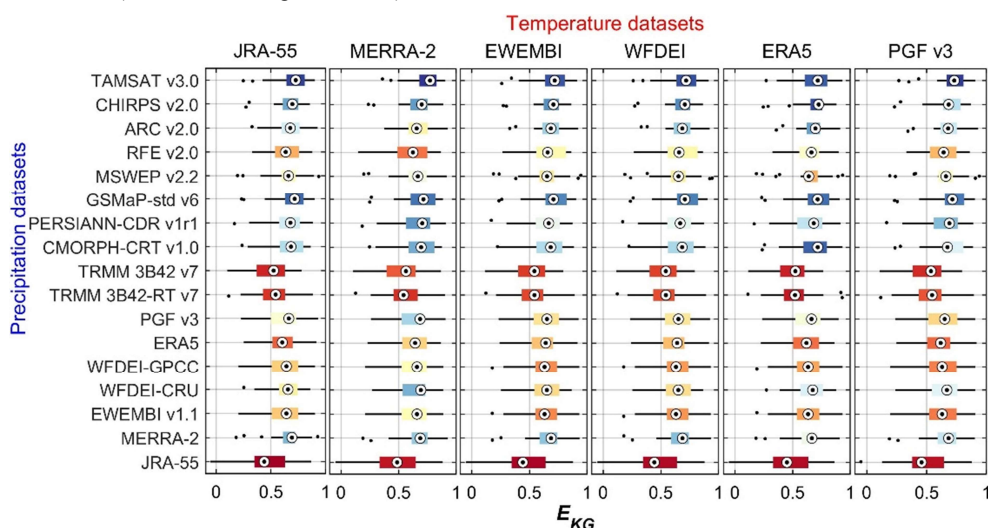
Figure 3. Kling-Gupta efficiency ( E_{KG} ) of daily streamflow ( Q ) over the simulation period (2003-2012) for 102 combinations of 17 rainfall datasets (y-axis) and 6 temperature datasets (subplots on x-axis) used as inputs in the mHM model. Each boxplot has 22 values representing the combined performance for the calibration and evaluation periods for 11 streamflow gauging stations. The boxplots are colored from the best (blue) to the worst performance (red) based on the median value.
