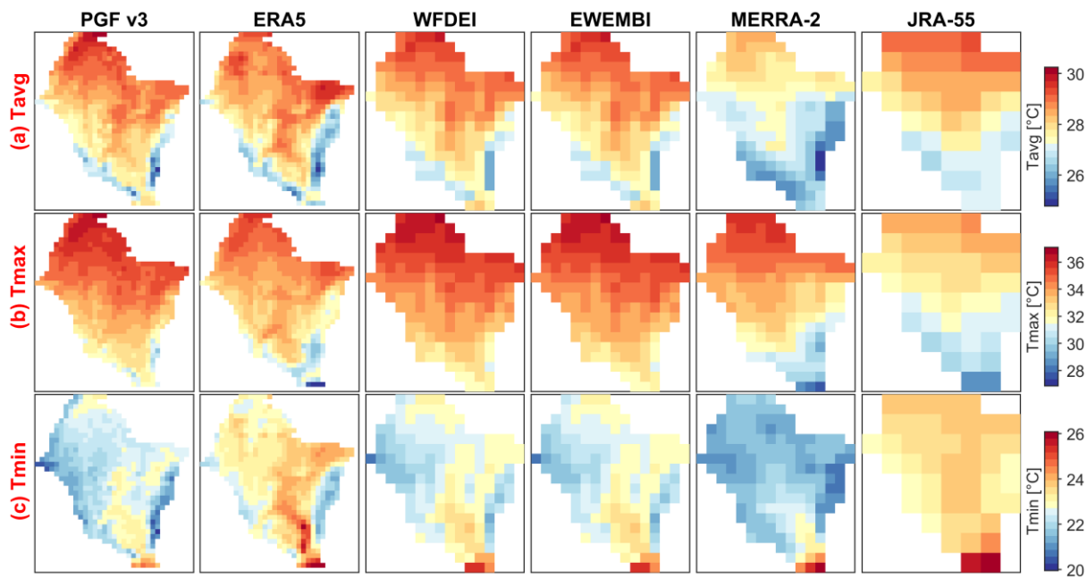
535 A2. Mean annual air temperature (average (a), maximum (b) and minimum (c)) over the period 2003-2012 for 6 temperature datasets in the Volta River basin
