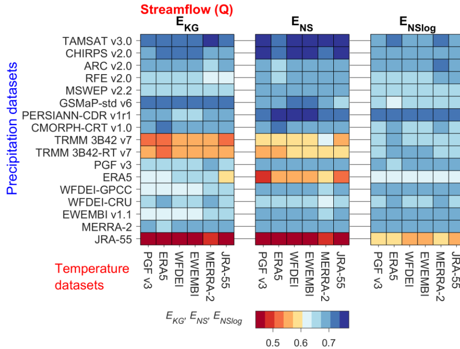
340 Figure 3. Kling-Gupta efficiency ( E_{KG} ), Nash-Sutcliffe efficiency ( E_{NS} ) and Nash-Sutcliffe efficiency of the logarithm ( E_{NSlog} ) of daily streamflow ( Q ) over the simulation period (2003-2012) for 102 combinations of 17 rainfall datasets (y-axis) and 6 temperature datasets (x-axis) used as forcing for the hydrological model.
