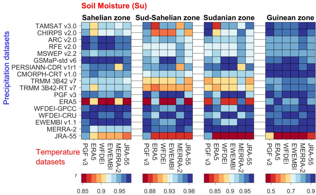
380 Figure 5. Pearson correlation coefficient ( r ) of modelled soil moisture ( S_u ) compared to ESA CCI data over the simulation period (2003-2012) considering 102 combinations of rainfall (y-axis) and temperature datasets (subplots on x-axis) used as forcing for the hydrological model.
