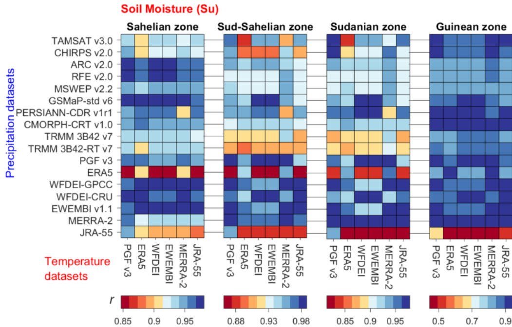
380 Figure 5. Pearson correlation coefficient ( r ) of modelled soil moisture ( S_u ) compared to ESA CCI data over the simulation period (2003-2012) considering 102 combinations of rainfall (y-axis) and temperature datasets (subplots on x-axis) used as forcing for the hydrological model.
