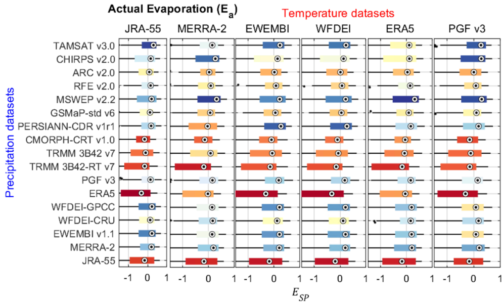
440 Figure 10. Spatial pattern efficiency ( E_{SP} ) of actual evaporation ( E_a ) over the entire simulation period (2003-2012) for the Volta River basin (VRB) using different combinations of precipitation and temperature datasets used as input for hydrological modelling. Each boxplot has 120 values corresponding to the number of months. The boxplots are colored from the best (blue) to the worst performance (red) based on the median value.
