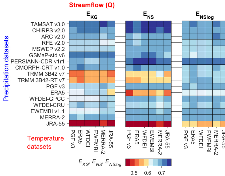
345 Figure 3. Kling-Gupta efficiency ( E_{KG} ), Nash-Sutcliffe efficiency ( E_{NS} ) and Nash-Sutcliffe efficiency of the logarithm ( E_{NSlog} ) of daily streamflow ( Q ) over the simulation period (2003-2012) for 102 combinations of 17 rainfall datasets (y-axis) and 6 temperature datasets (x-axis) used as forcing for the hydrological model.
