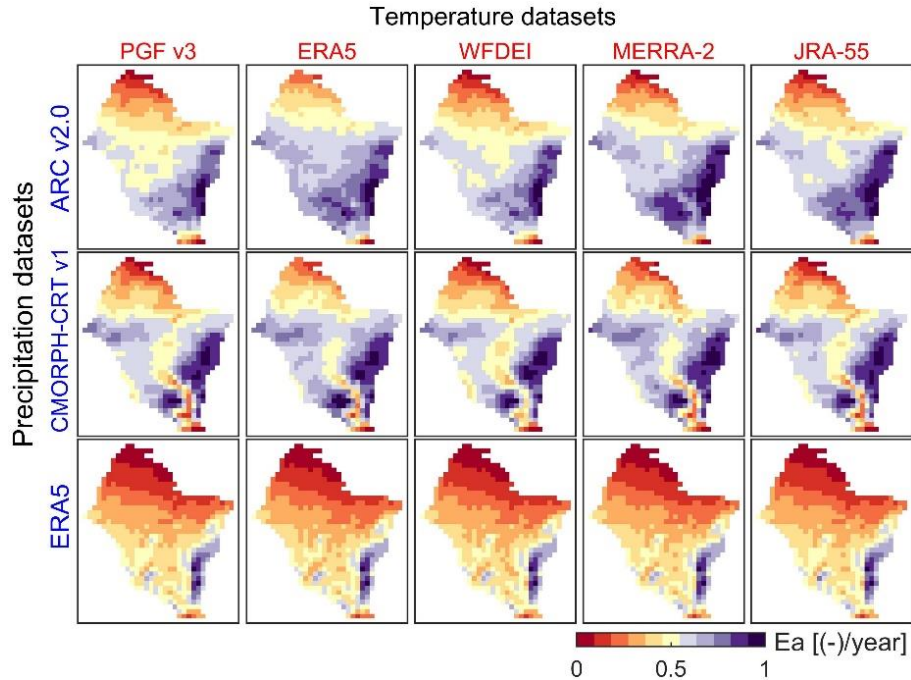
425 Figure 9. Maps of long-term (2003-2012) average of annual actual evaporation ( E_a ) obtained with different forcing of rainfall (y-axis, blue font) and temperature (x-axis, red font) datasets. The values are normalized between 0 and 1 to emphasize spatial patterns and to use a unique color scale.
