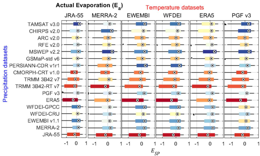
445 Figure 10. Spatial pattern efficiency ( E_{SP} ) of actual evaporation ( E_a ) over the entire simulation period (2003-2012) for the Volta River basin (VRB) using different combinations of precipitation and temperature datasets used as input for hydrological modelling. Each boxplot has 120 values corresponding to the number of months. The boxplots are colored from the best (blue) to the worst performance (red) based on the median value.
