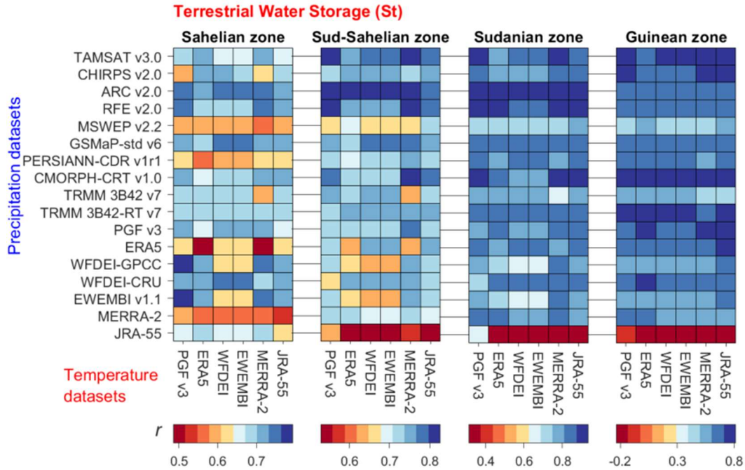
365 Figure 4. Pearson correlation coefficient ( r ) of modelled terrestrial water storage compared to GRACE data in four climatic zones in the Volta River basin over the simulation period (2003-2012) considering 102 combinations of rainfall (y-axis) and temperature datasets (subplots on x-axis) used as forcing for the hydrological model.
