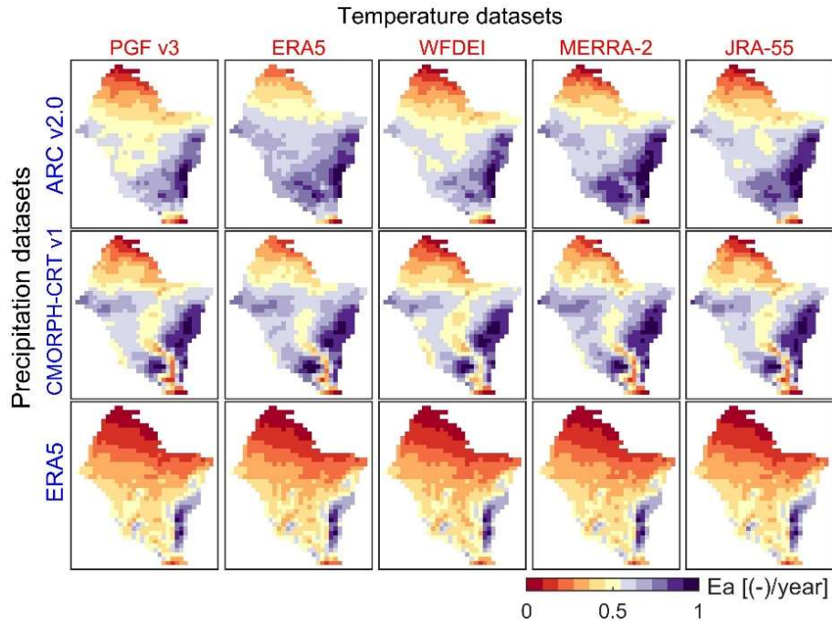
430 Figure 9. Maps of long-term (2003-2012) average of annual actual evaporation ( E_a ) obtained with different forcing of rainfall (y-axis, blue font) and temperature (x-axis, red font) datasets. The values are normalized between 0 and 1 to emphasize spatial patterns and to use a unique color scale.
