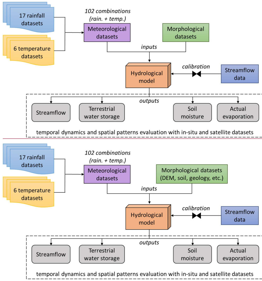
Figure 1. Flowchart of the methodology used to evaluate the suitability of meteorological datasets in reproducing plausible hydrological processes.
