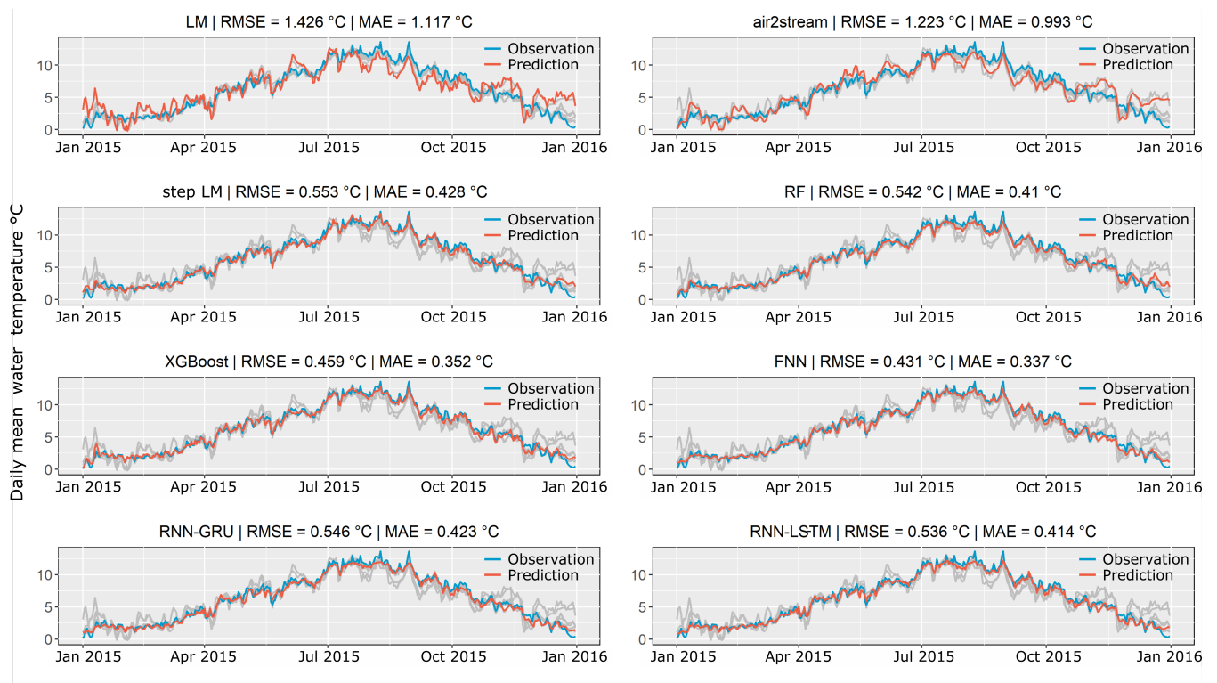
Figure 5. Comparison of the prediction of all tested model types for the Inn catchment for the year 2015. Data from 2015 was not used for training and validation. Prediction results for each model are shown with red lines, while the observations are shown in blue lines. The predictions of all other models are illustrated with grey lines.
