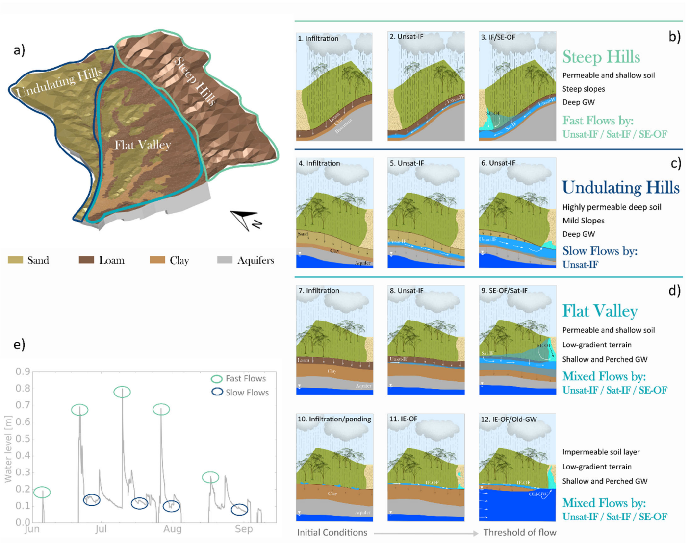
Figure 3: a) Conceptual diagram showing the three major areas that are likely to develop distinct streamflow generation mechanisms during the intermittent flow season. b-d) 2D soil profiles for the three major areas detailing the processes developing from the initial conditions until the threshold of flow (modified from Gutierrez-Jurado et al., 2019) e) Typical hydrograph during the intermittent season highlighting the hypothesized ‘fast’ and ‘slow’ flow components.
