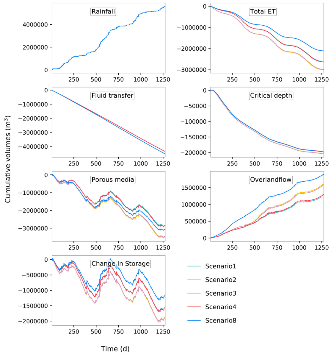
785 Figure 6: Cumulative values of the water balance components simulated with HydroGeoSphere for scenarios 1-4 and 8.
