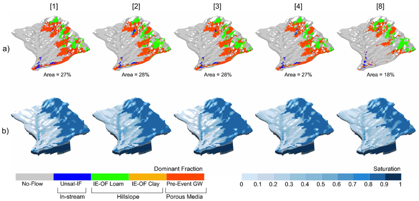
780 Figure 5: Snapshots of time step 960 during a rainfall event showing (a) the spatial extent of active areas by their dominant HMC component (flow generation mechanism) for each scenario (1-4 and 8) and (b) the porous media saturation. The spatial extent of active areas as a percentage of the catchment area is shown below the snapshots. Colours for the HMC components show both the dominant process and the origin of the water contributing to the flow in each cell. For example, all red areas are from Pre-event GW some of which can contribute to active areas in both the stream and in the stream banks.
