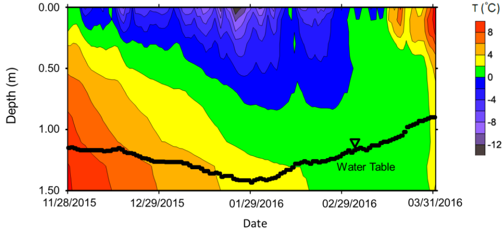
Figure 2. The contour map showing the evolution of soil temperature at the study site during the freezing-thawing cycle. Also shown is the monitored fluctuating groundwater level.
