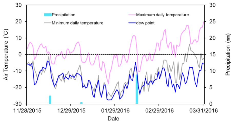
Figure 3 The maximum daily air temperature, the minimum daily air temperature, dew-point temperature and precipitation during the freezing-thawing cycle from 28 NOV 2015 to 1 APR 2016.
