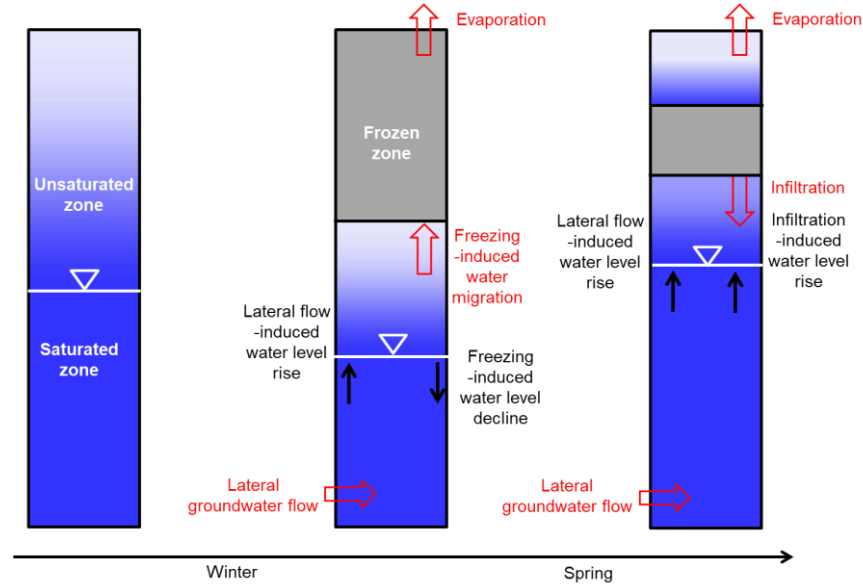
Figure 1 The conceptual model showing main hydrological and hydrogeological processes in semi-arid regions during the freezing-thawing cycle.
