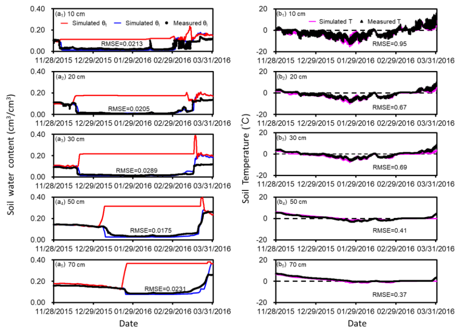
Figure 5 The observed and simulated liquid water content and simulated total water content ( \theta_l ) (a 1 -a 5 ) and soil temperature (b 1 -b 5 ) at the 5 different depths within the frozen zone during the freezing-thawing cycle. The RMSEs of liquid water content and soil temperature are also listed.
