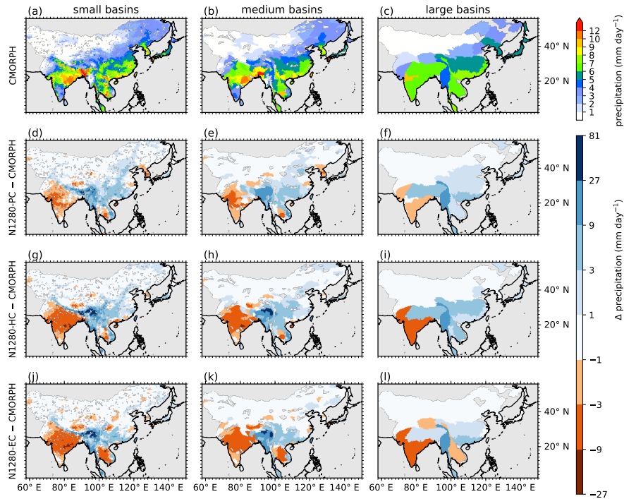
Figure 4. Mean JJA precipitation over Asia averaged over basins of different scales showing CMORPH (top), and difference between simulations and CMORPH for N1280-PC (middle second row), N1280-HC (third row) and N1280-EC (bottom). One basin scale is shown in each column, and one dataset is shown in each row. Areas shown in grey are not covered by selected basins (see Sects. 2.4.1 and 2.4.2).
