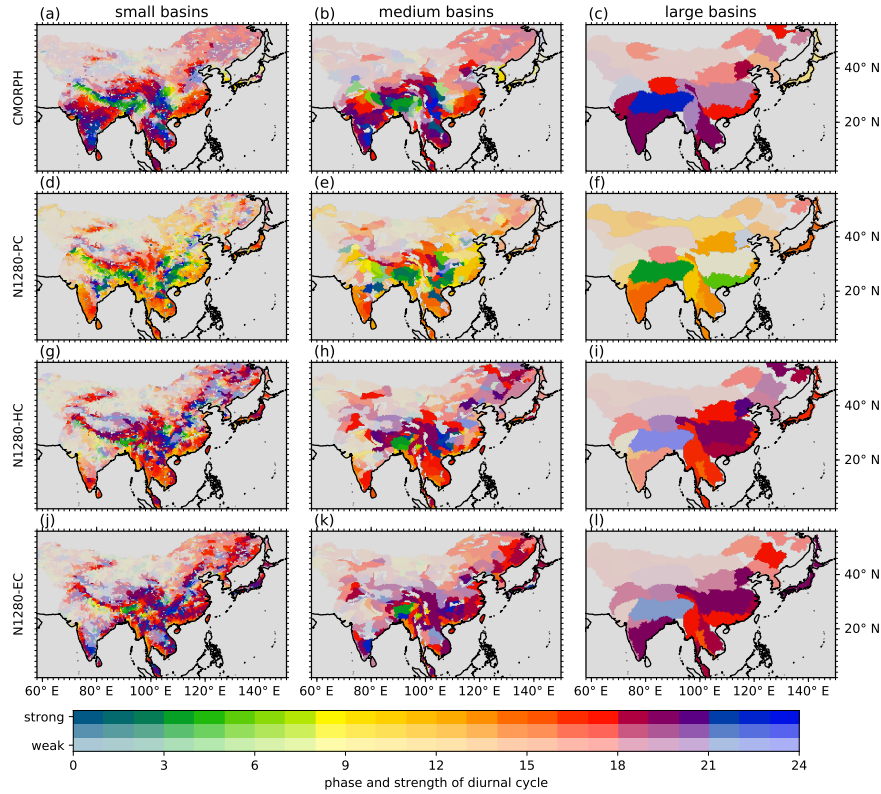
Figure 7. Amount-Diurnal cycle of amount of precipitation over Asia averaged over different basin scales (columns) for CMORPH, N1280-PC, N1280-HC and N1280-EC (rows). As described in Sect. 2.3 and as in Fig. 10, a visual representation of the amplitude is given by its strength, dependent on whether it is strong, medium or weak. This is calculated separately for each dataset and scale (i.e. for each panel).
