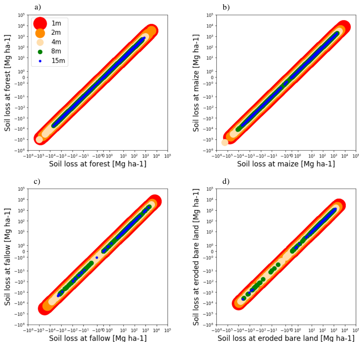
450 Figure 13. Cumulative soil loss ( \text{Mg ha}^{-1} ) of: (a) forest, (b) maize, (c) fallow, and (d) eroded bare land cover across resolutions.
