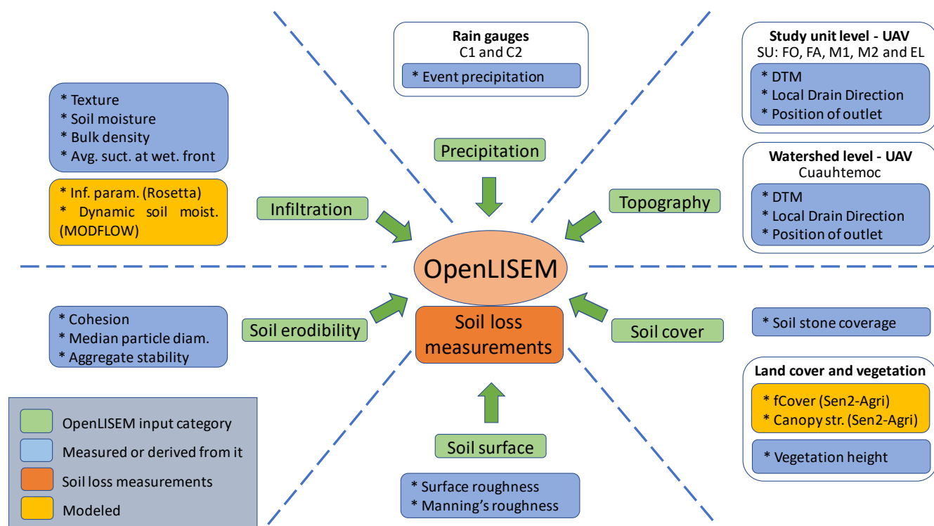
Figure 3. Overview of measured / derived input data used for modelling. Soil loss measurements on the ground were used for model validation.
