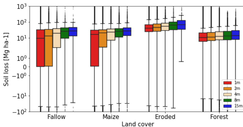
Figure B2. Cumulative soil loss (Mg ha -1 ) box-plot per land cover across resolutions
