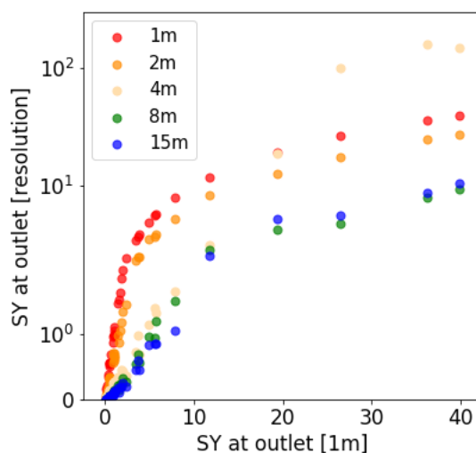
410 Figure 11. Event sediment yield (SY) at watershed outlet across resolutions.
