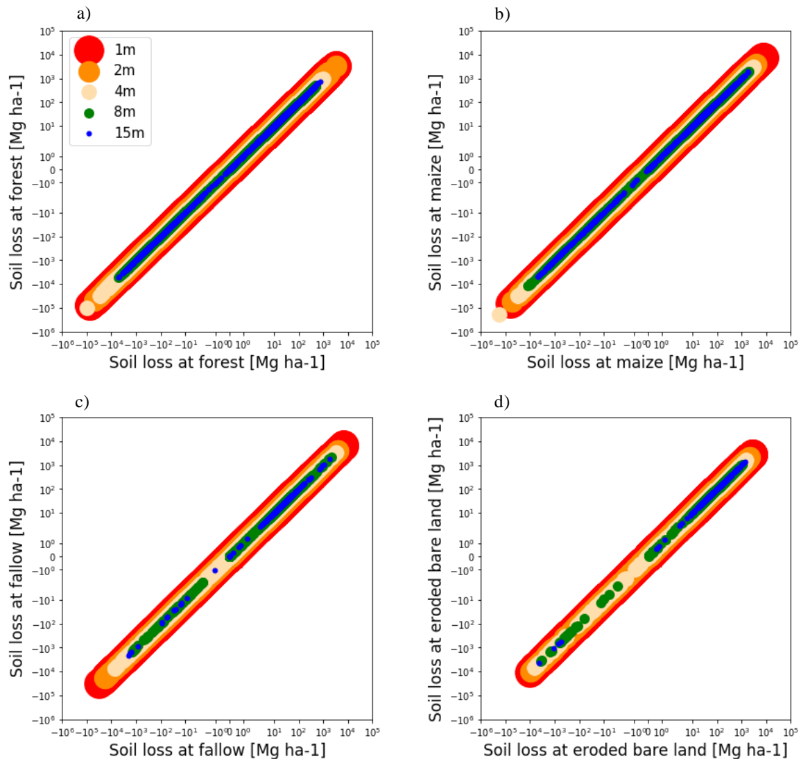
Figure 13. Cumulative soil loss (Mg ha -1 ) of: (a) forest, (b) maize, (c) fallow, and (d) eroded bare land cover across resolutions.
