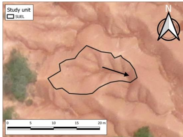
175 Figure 2. Study unit set up: (a) SUFO (forest), (b) SUFA (fallow), (c) SUM1 (maize), (d) SUM2 (maize), and (e) SUEL (eroded bare land). Arrows indicate the main flow direction. Image source: 2016 UAV flight campaign.
