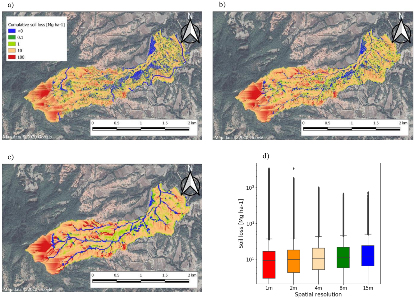
440 Figure 12. Cumulative soil loss ( \text{Mg ha}^{-1} ) during the collection period at: (a): 1 m, (b): 4 m, (c): 15 m resolution, and (d) box-plot per resolution.
