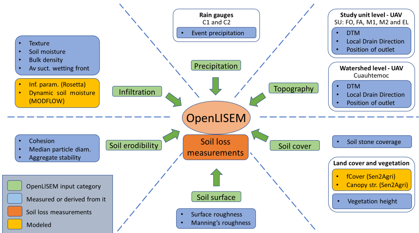
205 Figure 3. Overview of measured / derived input data used for modelling. Soil loss measurements on the ground were used for model validation.
