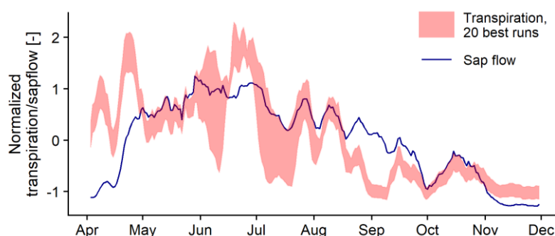
Figure 7: Measured sap flux density (average of six trees, blue line) and simulated transpiration (red envelop). Both time series were normalized and smoothed with a seven-day moving average to facilitate visual comparison.
