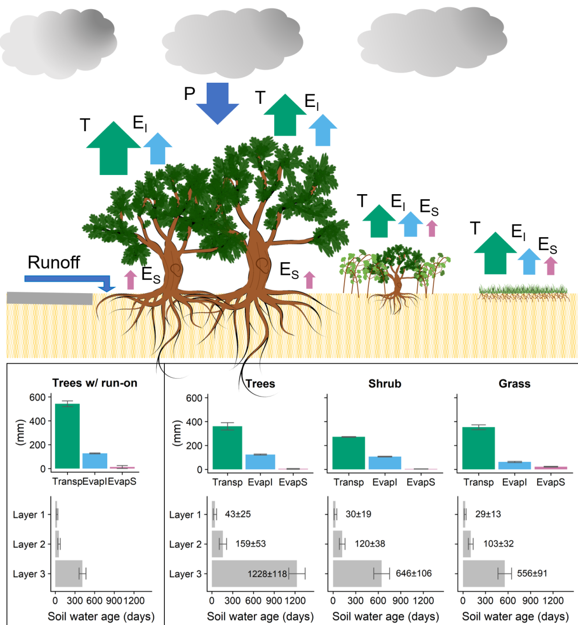
Figure 10: Conceptualisation of the simulation results: ecohydrological fluxes and ages over the growing season at the SUEO 2019. Transpiration (T, green), interception evaporation (E i , light blue), soil evaporation (E s , pink), precipitation (P) and surface runoff (dark blue).
