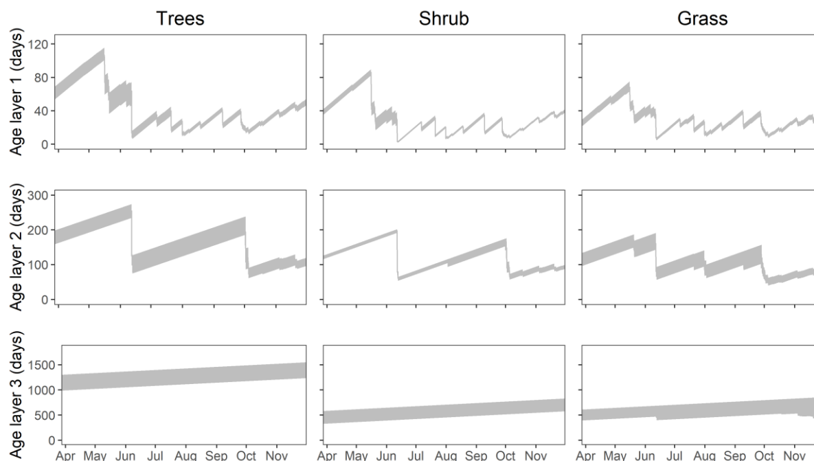
Figure 9: Modelled water ages (days) in soil layers 1, 2 and 3 under trees, shrub and grass.
