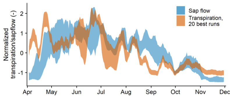
320 Figure 7: Measured sap flux density (average of six trees, blue line) and simulated transpiration (red envelop). Both time series were normalized and smoothed with a seven-day moving average to facilitate visual comparison.
