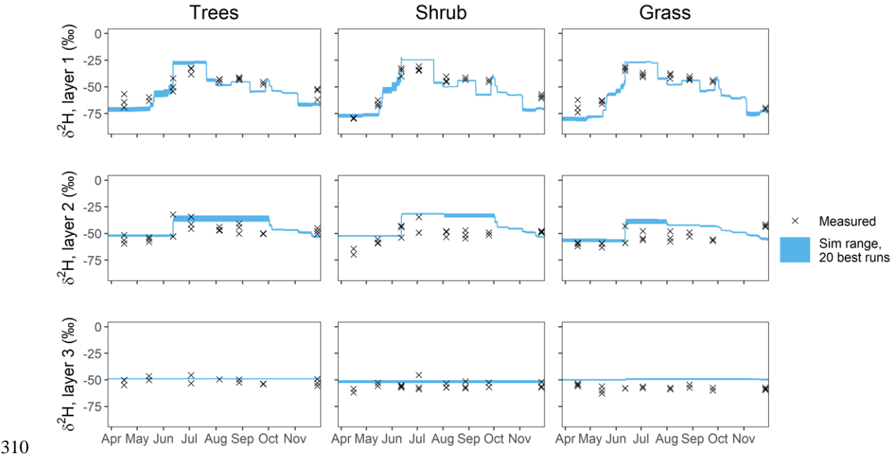
310 Figure 6: Measured and simulated stable water isotope \delta^2\text{H} in bulk soil water. KGE values given for layer 1.
