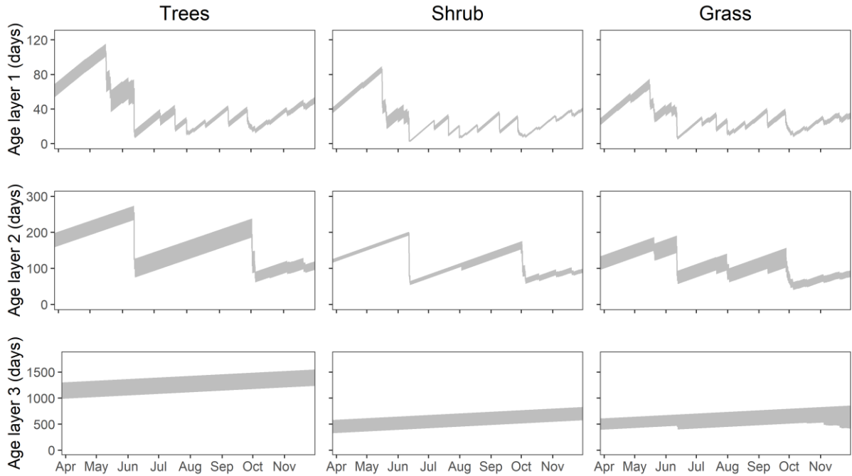
Figure 9: Modelled water ages (days) in soil layers 1, 2 and 3 under trees, shrub and grass.
