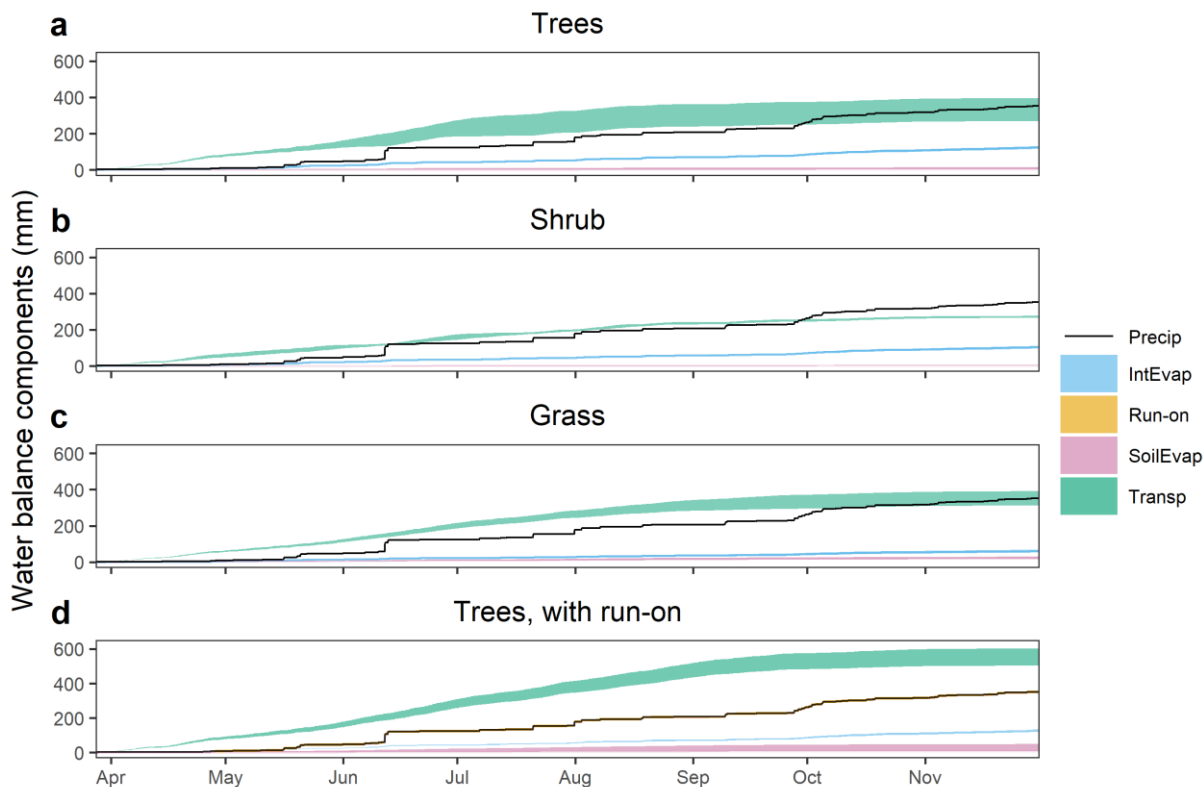
Figure 8: Cumulative precipitation (Precip), evaporation from intercepted water (IntEvap), run-on, evaporation from soil water (SoilEvap) and transpiration (Transp) for trees (a), shrub (b), grass (c) and trees with run-on from adjacent sealed surface (d).
