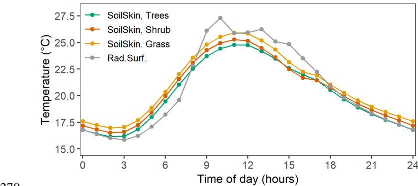
Figure 4: Diurnal summer (June to August) temperature cycles. Modelled soil skin temperature (SoilSkin, average of 20 best runs) for all vegetation types (trees, shrub and grass) and calculated radiative temperature (Rad.Surf.) from upward longwave radiation.
