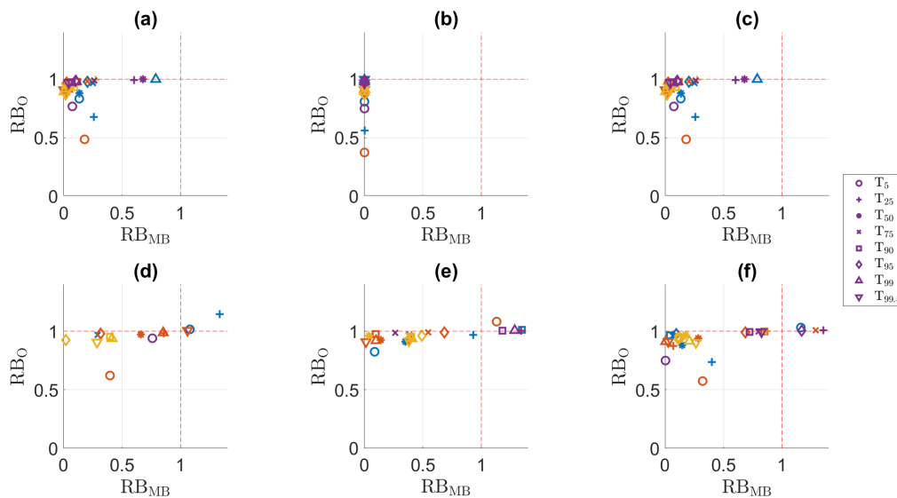
Figure 4. RB_{MB} versus RB_0 for the temperature indices in the calibration period. (a) QDM, (b) mQDM, (c) MBCn, (d) MRQNBC, (e) dOTC, (f) R 2 D 2 . Winter: blue, spring: ochre, summer: yellow, autumn: purple.
