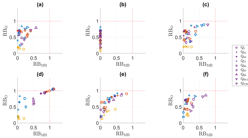
Figure 10. RB_{MB} versus RB_0 for the discharge percentiles and the 20-year return period value in the calibration period. (a) QDM, (b) mQDM, (c) MBCn, (d) MRQNBC, (e) dOTC, (f) R^2D^2 . Winter: blue, spring: ochre, summer: yellow, autumn: purple.dr
