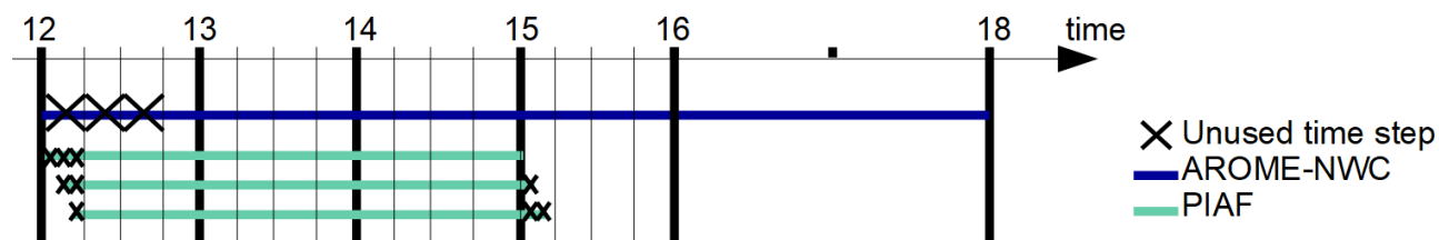
Figure 2. Example showing the unused time steps for an AROME-NWC forecast run starting at 1200 UTC and for three successive PIAF forecasts starting at 1200, 1205 and 1210 UTC.
