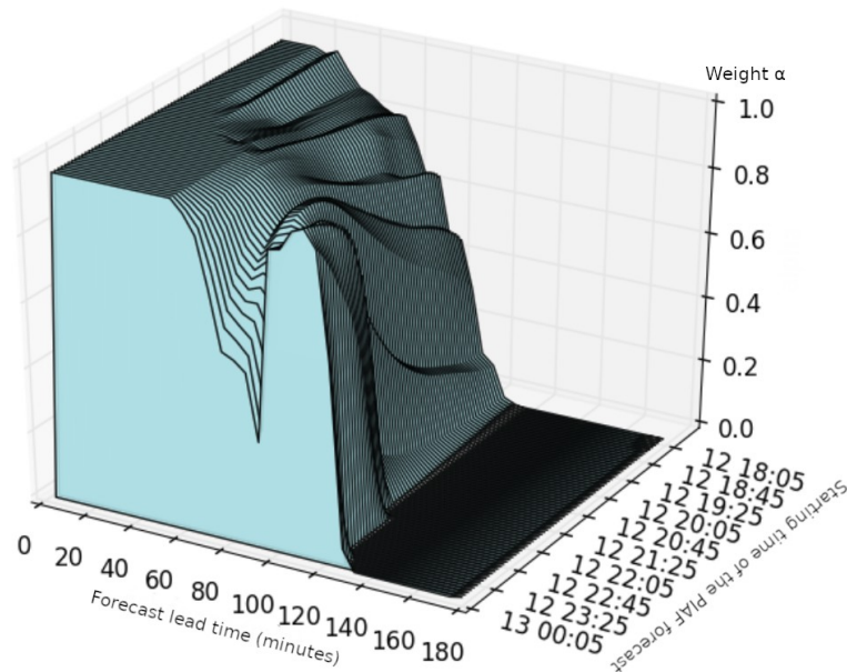
Additional figure : 3-D representation of the weight \alpha given to radar extrapolation in PIAF. It shows the PIAF forecast lead time (interval [0, 180 minutes]) dependency on \alpha (interval [0, 1]) for PIAF forecasts starting from 12 October 2016 18:05UTC to 13 October 2016 00:05UTC.
