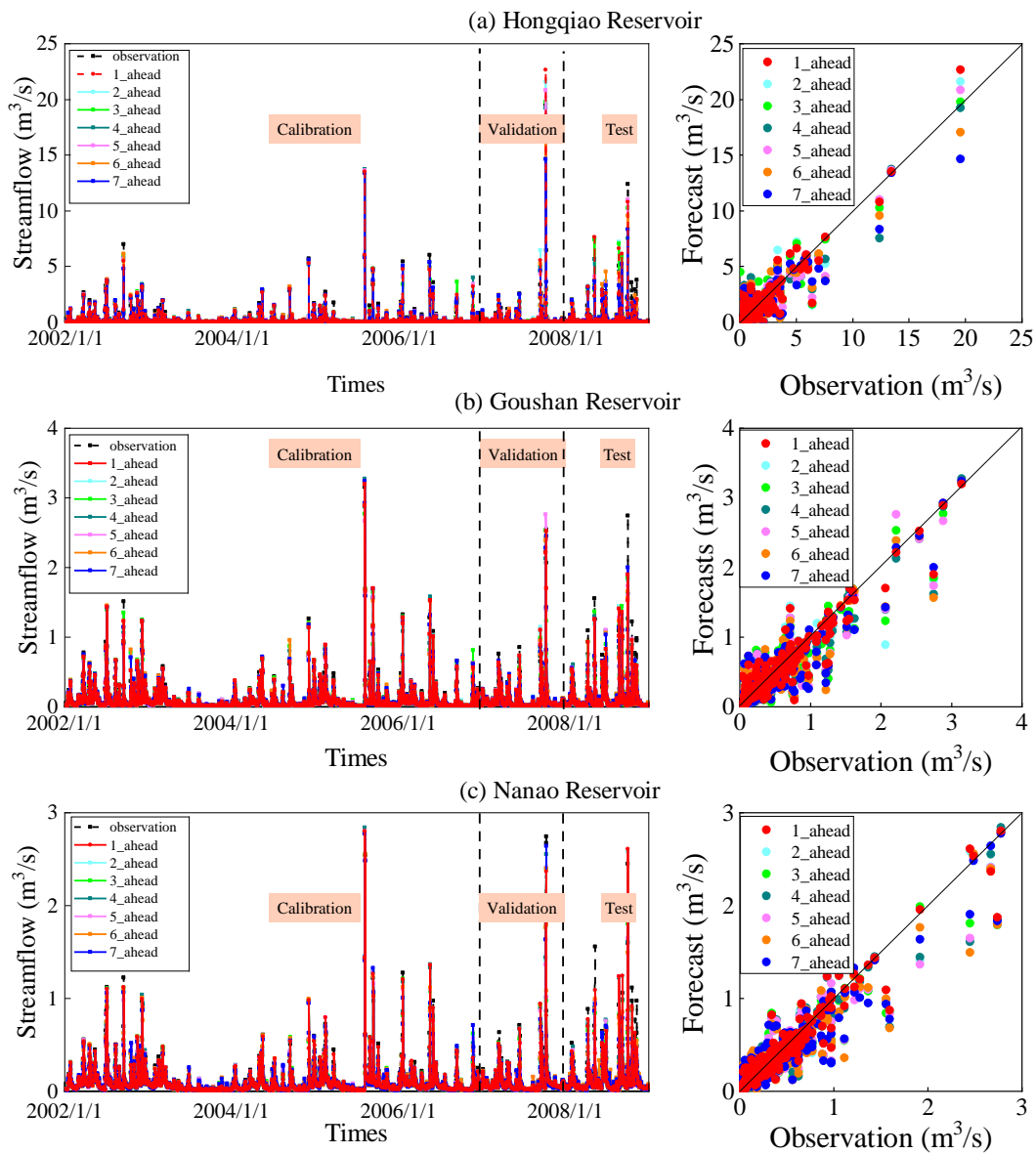
895 Figure 11: Forecast results of (a) Hongqiao, (b) Goushan, and (c) Nanao reservoirs under S5.
