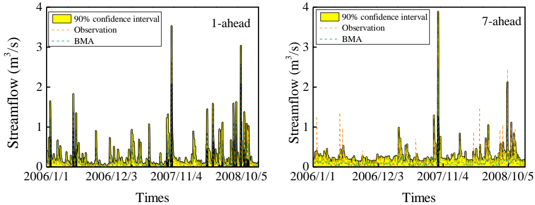
Figure 12: 90% streamflow interval of the BMA method under S3.
