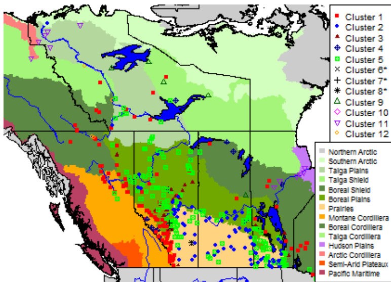
1695 Figure 7. Locations of the 12 Streamflow Regime Types from the changing cold regions domain overlain on the ecosystems of western Canada. Clusters marked with an * have only a single member.
