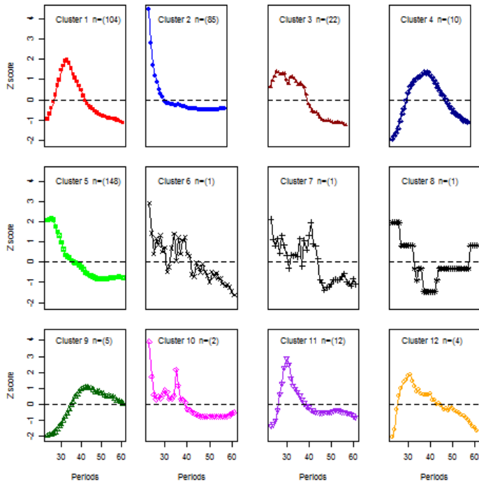
1700 Figure 8. Centroids of the 12 Streamflow Regime Type clusters.
