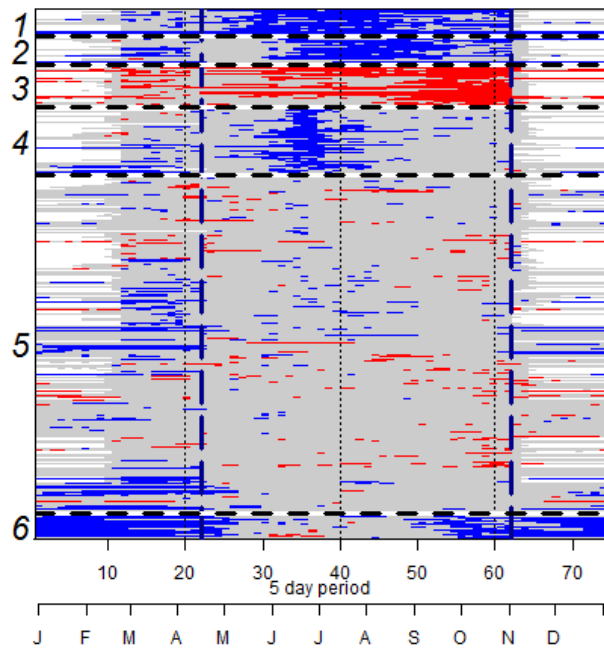
Figure 10. Trend Patterns in the 395 stations, significant increases (blue) and significant decreases (red), no trend (gray) and missing (white). The stations are ordered by Trends Pattern (cluster) number and stationID. Data outside the dashed lines was not used in the clustering, but is shown where available (periods 1-22 and 62-73).
