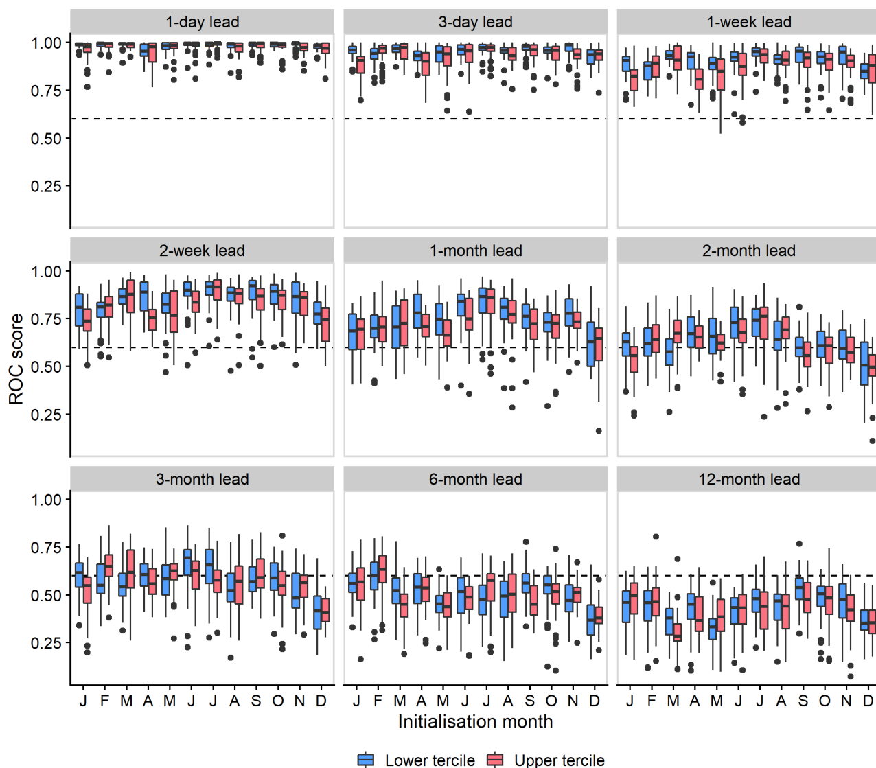
Figure 8. Distribution of ROC score values across all 46 study catchments for each initialisation month (January to December) and the same selection of lead times as in Fig. 5. Forecasts are considered skilful if the ROC score > 0.6 .
