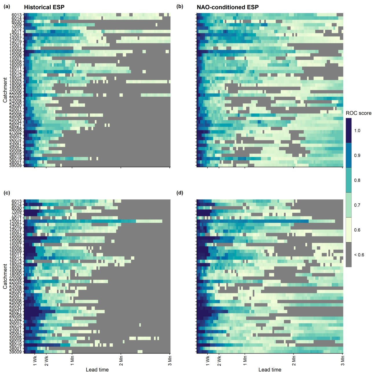
Figure 10. Comparison of ROC scores achieved by historical ESP (left) and NAO-conditioned ESP (right) across all 46 study catchments and all lead times for low flow (lower tercile, a–b) and high flow (upper tercile, c–d) events.
