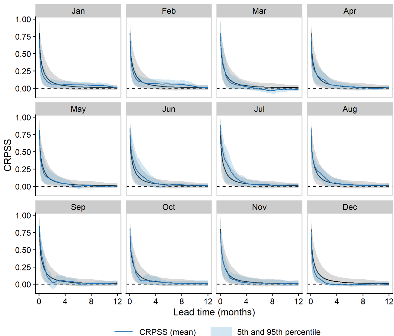
Figure 4. As in Fig. 3, but for each forecast initialisation month. Data from Fig. 3 is included in the background of each panel for reference.
