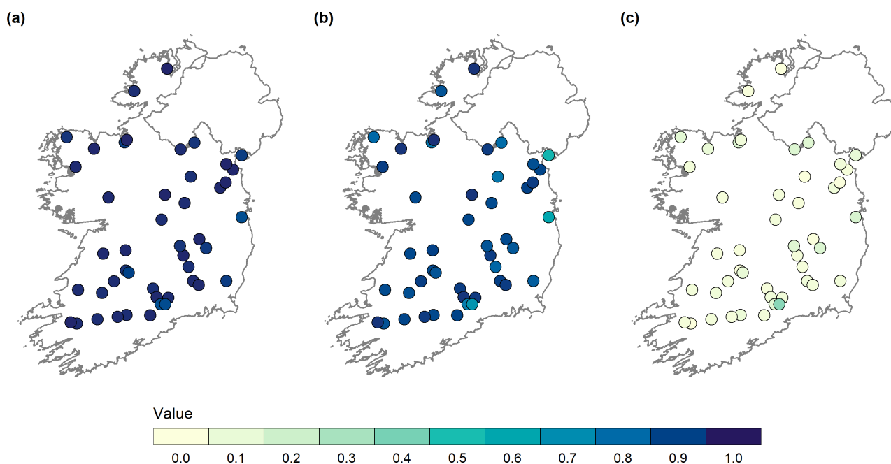
Figure 2. GR4J model performance over the complete period (1993–2017) as measured by (a) KGE_{NP} , (b) NSE, and (c) absolute PBIAS.
