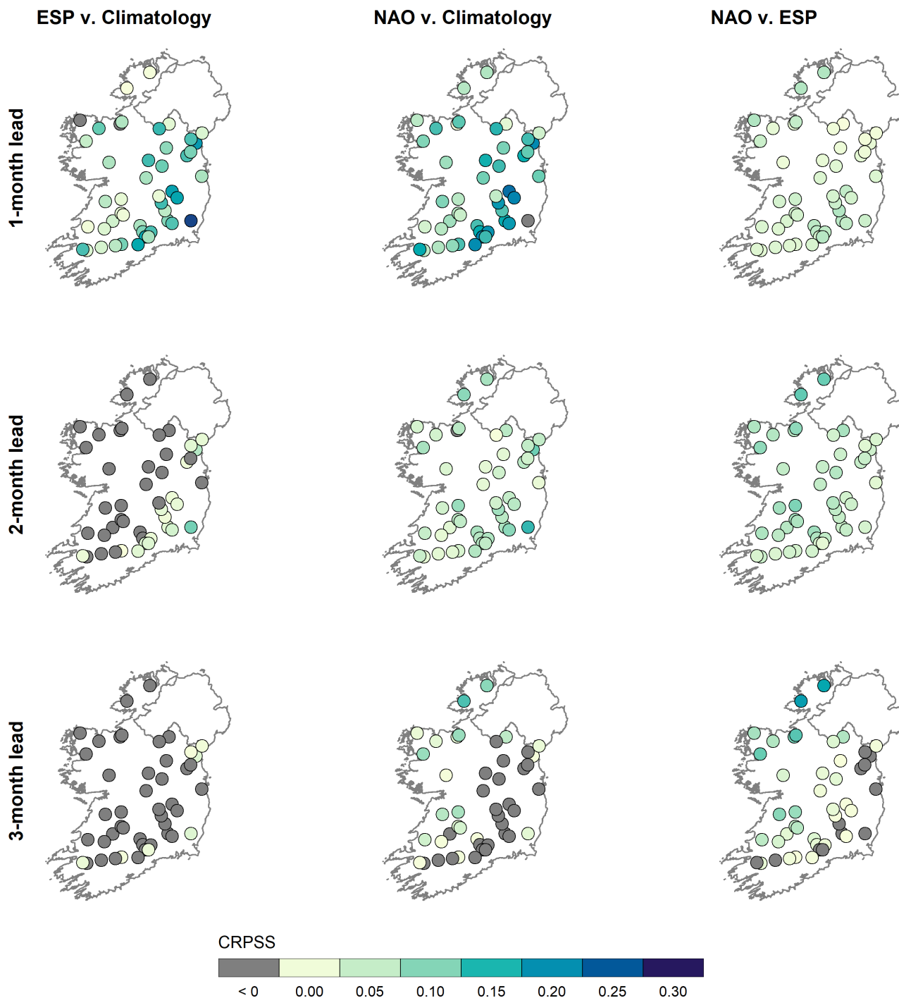
Figure 9. CRPSS values for historical ESP (left), NAO-conditioned ESP (middle), and the improvement made by NAO-conditioned ESP over historical ESP (right), at lead times of 1, 2, and 3 months.
