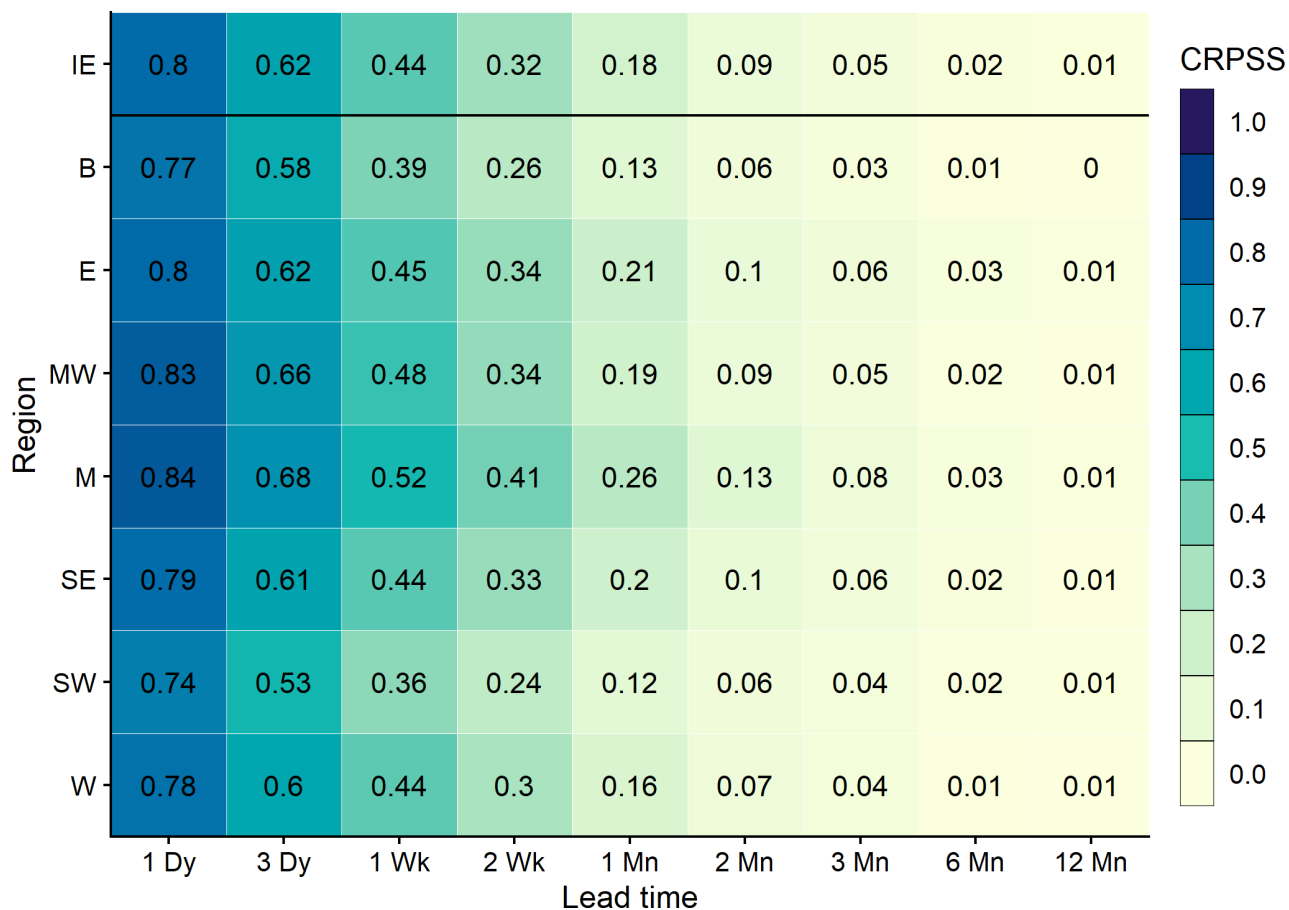
Figure 5. CRPSS values for Ireland (IE) and seven NUTS III regions (B, E, MW, M, SE, SW, and W) averaged across all initialisation months for a selection of lead times: short (1- and 3-day), extended (1- and 2-week), monthly (1- and 2-month), seasonal (3- and 6-month) and annual (12-month).
