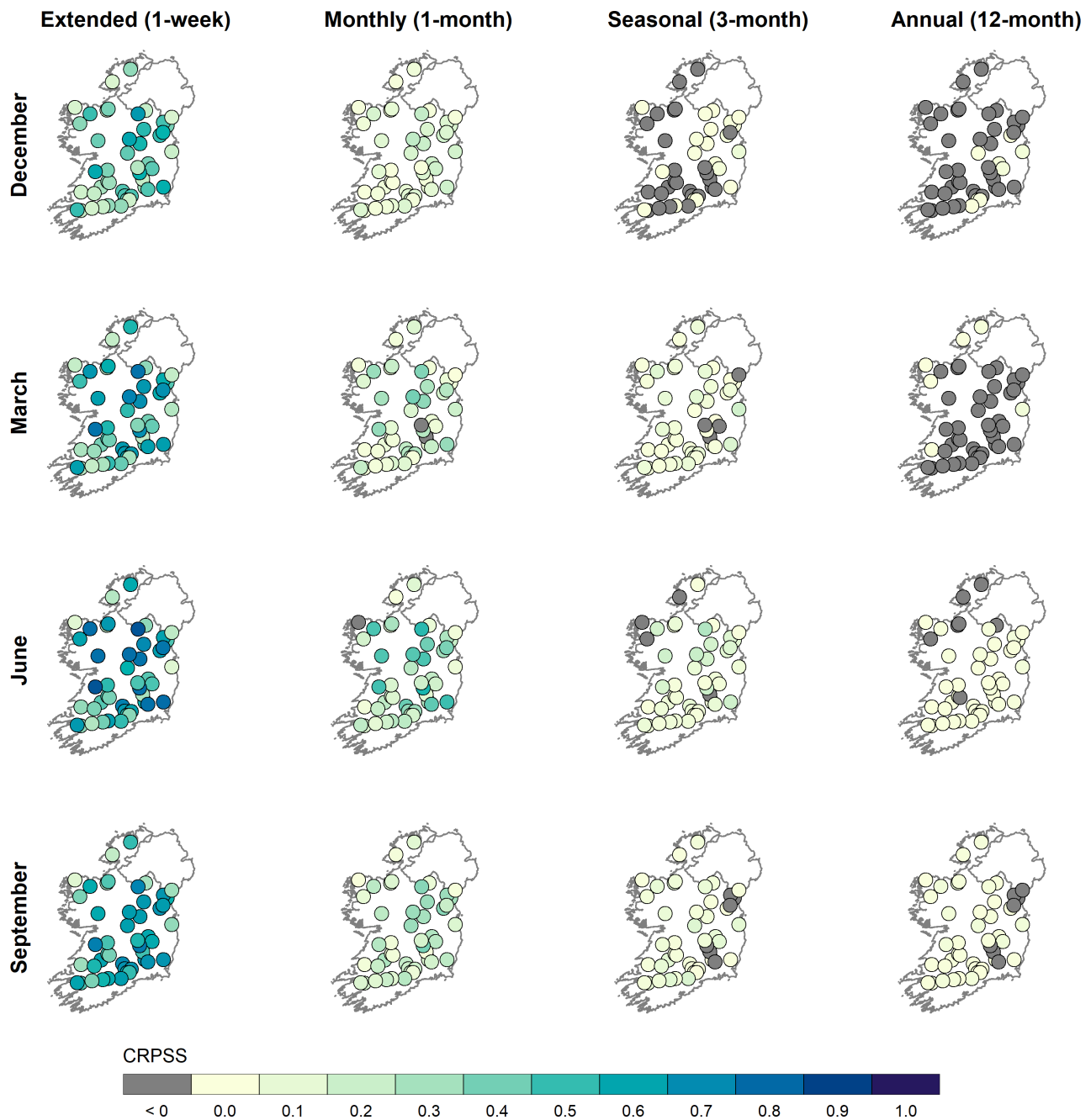
Figure 6. ESP skill for individual forecasts made at the 46 catchments for four sample lead times (columns) and four initialisation months (rows).
