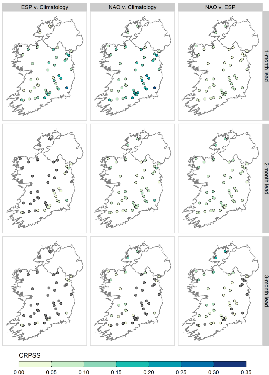
Figure 10. CRPSS values for historical ESP (left), NAO-conditioned ESP (middle), and the improvement made by NAO-conditioned ESP over historical ESP (right), at lead times of 1, 2, and 3 months. Catchments with negative skill (CRPSS < 0) are greyed out.
