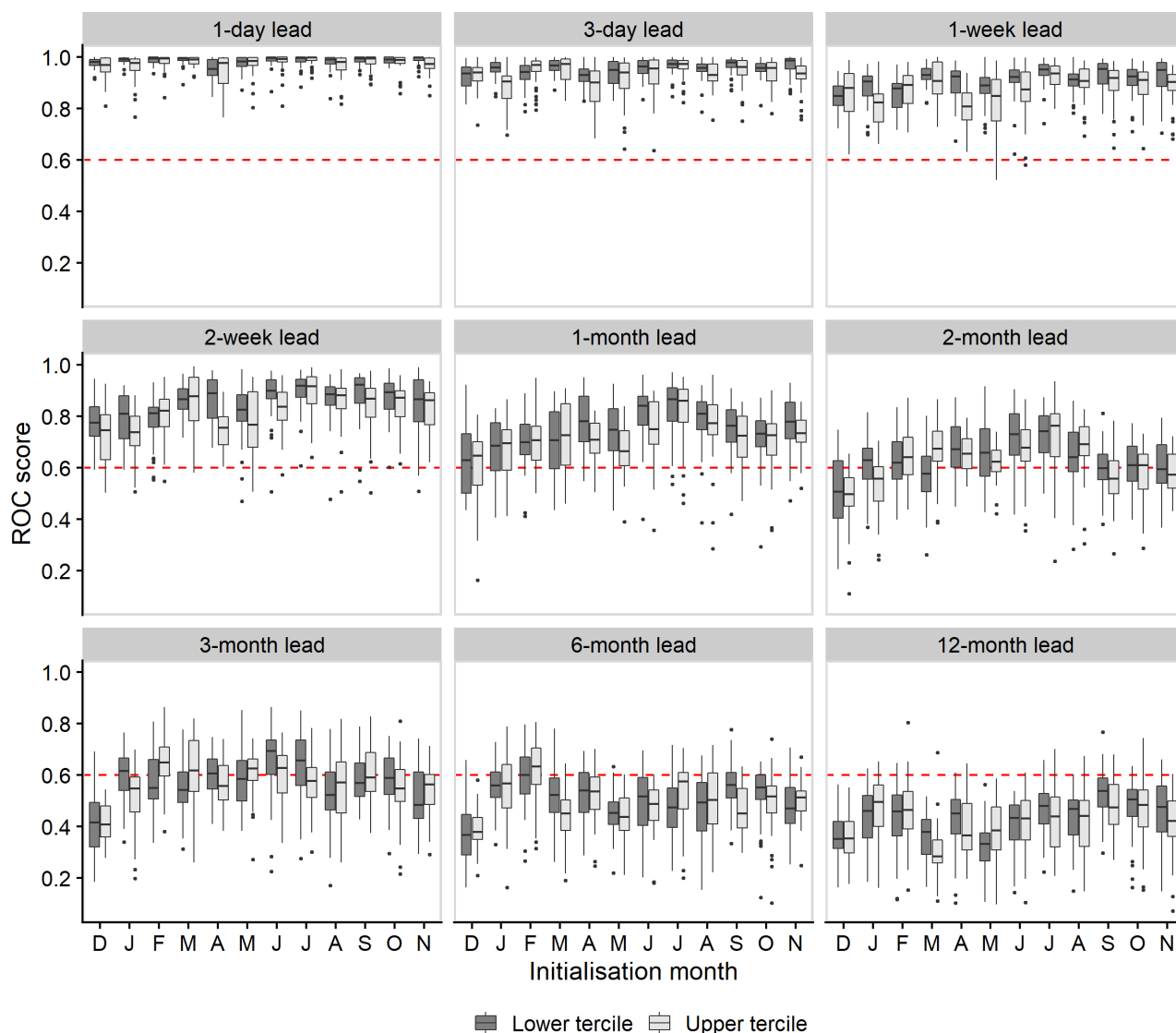
Figure 9. Distribution of ROC score values across all 46 study catchments for each initialisation month (January to December) and the same selection of lead times as As in Fig. 5. Forecasts are considered skilful if 8, but for the ROC score >. The red line denotes the stricter skill threshold of 0.6.
