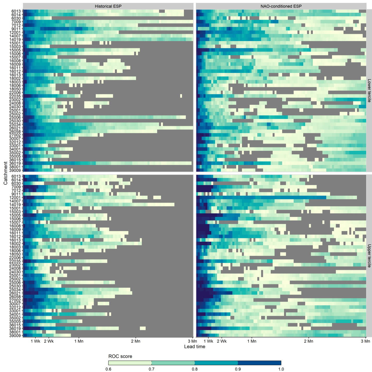
Figure 12. Comparison of ROC scores achieved by historical ESP (left column) and NAO-conditioned ESP (right column) across all 46 study catchments and all lead times for low flow (lower tercile, a-b upper row) and high flow (upper tercile, c-d lower row) events.
