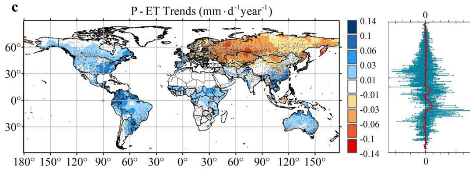
Figure 4. Long-term trends in evaporative fraction (EF), evapotranspiration (ET), and precipitation (P) minus ET (P-ET). ET was converted from the ANN retrieved latent heat flux. The red curve represents median trends at different latitudes.
