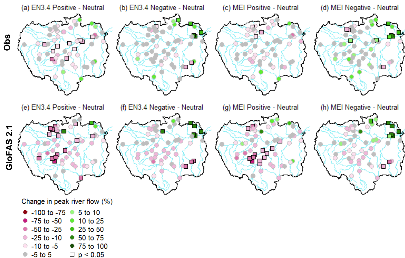
Figure 2. Percentage change of observed and simulated mean annual peak river flows between different phases of the EN3.4 and MEI indices, for (a, c, e, g) positive with respect to neutral years and (b, d, f, h) negative with respect to neutral years. Top row represents changes for observations, bottom row shows changes for GloFAS 2.1 streamflow reanalysis data. Pink (green) points represent where the average annual peak flow decreases (increases). Significant results at the 95 % confidence level are denoted using a square (i.e. p < 0.05 ).
