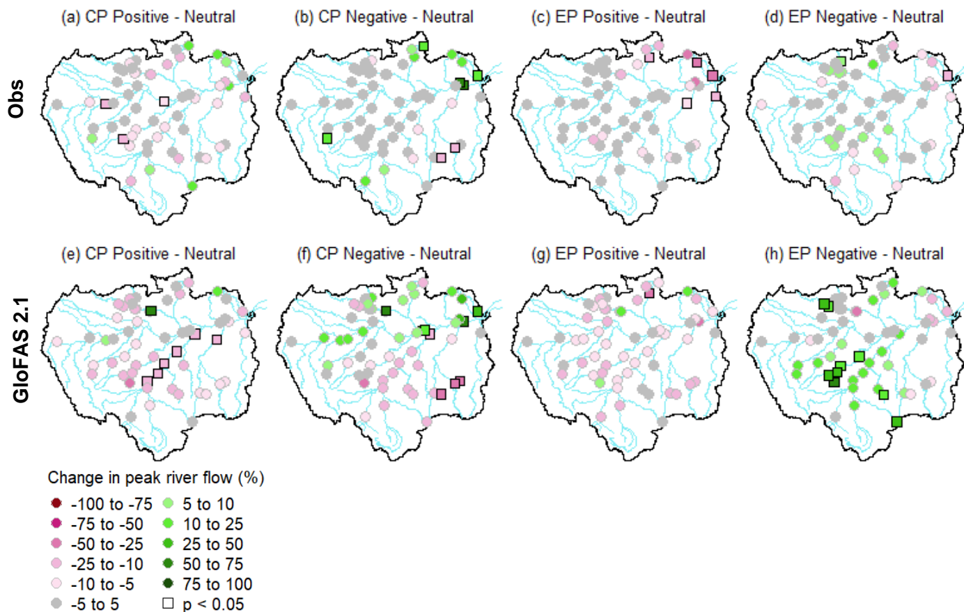
Figure 3. Percentage change of observed and simulated mean annual peak river flows between different phases of the CP and EP indices, for (a, c, e, g) positive with respect to neutral years and (b, d, f, h) negative with respect to neutral years. Top row represents changes for observations, bottom row shows changes for GloFAS 2.1 streamflow reanalysis data. Pink (green) points represent where the average annual peak flow decreases (increases). Significant results at the 95 % confidence level are denoted using a square (i.e. p < 0.05 ).
