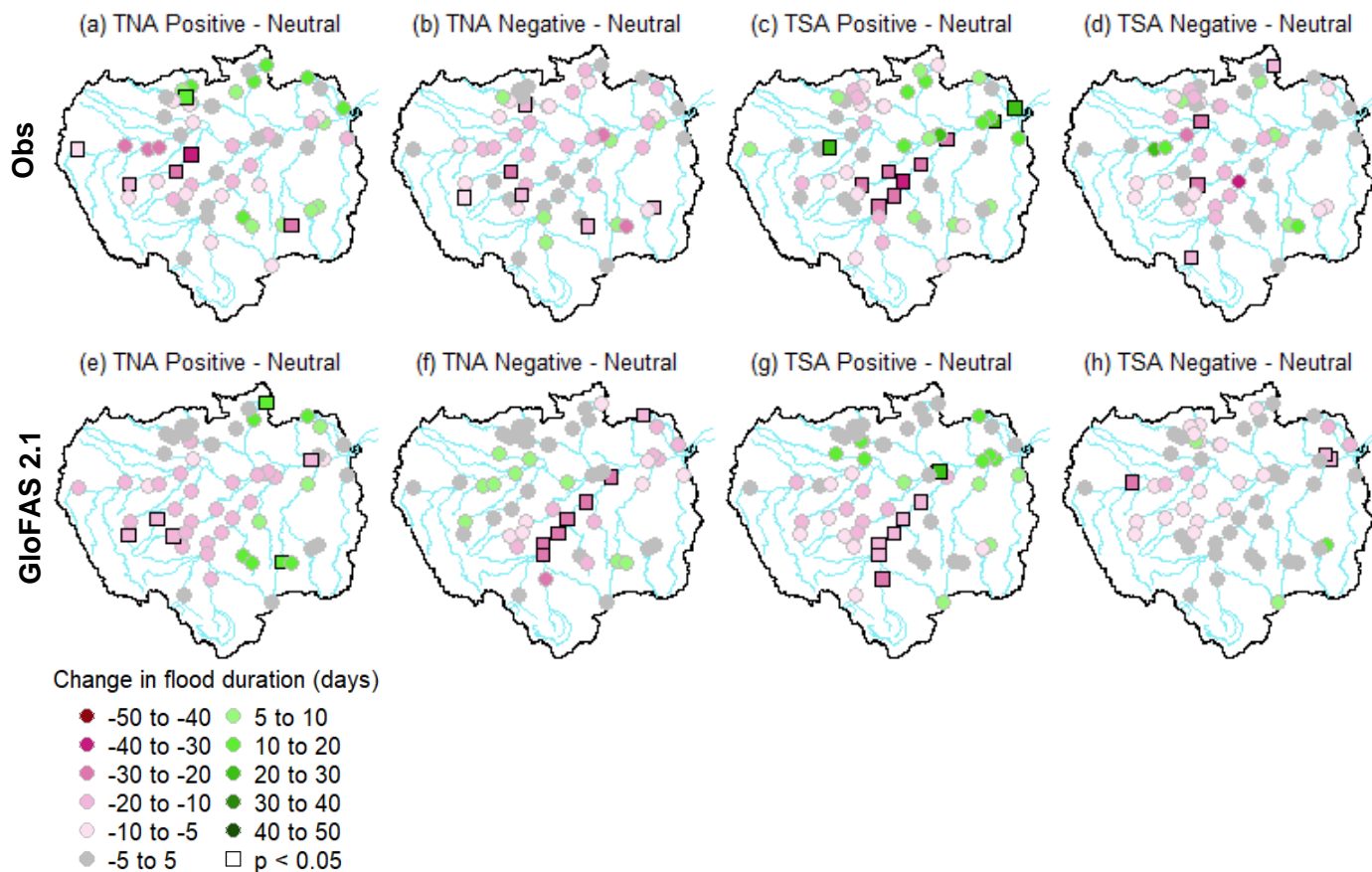
Figure 10. Changes in flood duration (i.e. mean number of days river flows exceed the 95 th percentile of each stations/grid point climatology) for different phases of tropical Atlantic indices. For (a, c, e, g) positive with respect to neutral years. (b, d, f, h) Negative with respect to neutral years. Top row represents changes for observations, bottom row shows changes for GloFAS 2.1 streamflow reanalysis data. Pink (green) points represent decreases (increases) in the number of days spent above the 95 th percentile compared to neutral conditions. Significant results at the 95 % confidence levels are denoted using a square (i.e. p < 0.05 ).
