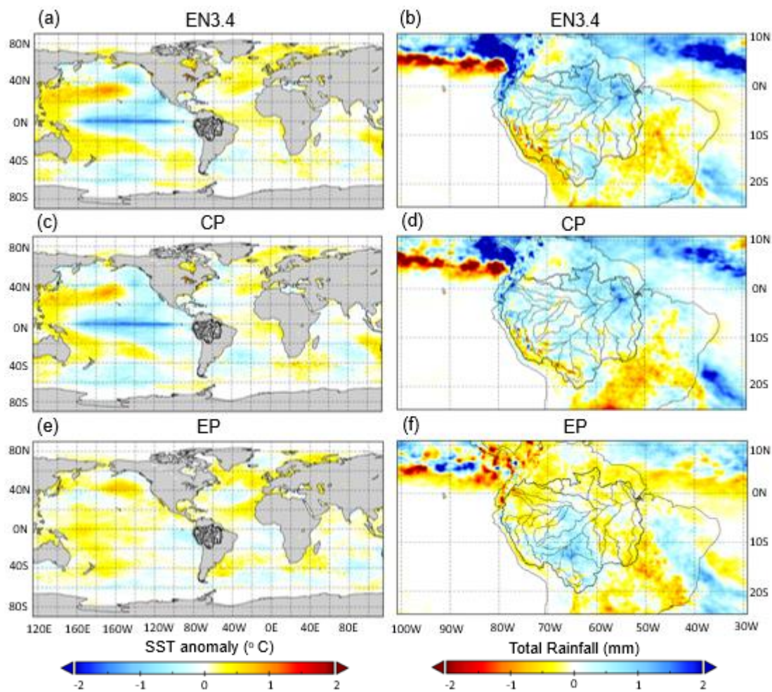
20 Figure 12. Composite analysis of the difference between the preceding OND average SST ( ^{\circ}\text{C} ) ( left ) and total rainfall (mm) ( right ) for the average of the 12 negative years and the average of the 12 neutral years. For the (a, b) EN3.4, (c, d) CP, and (e, f) EP indices. A list of the negative and neutral years for each index can be found in Tables S2, 4, and 5.
