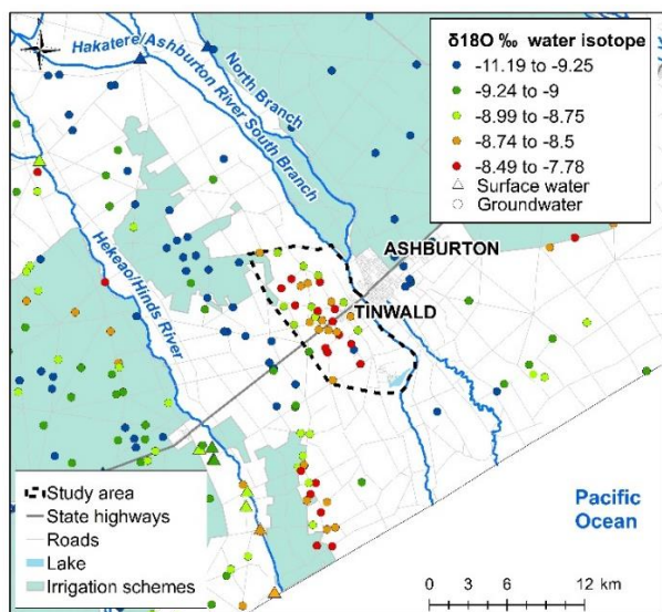
Figure 6: \delta^{18}\text{O} in the Ashburton area at groundwater and surface water sites. Data outside of the Tinwald study area is mean \delta^{18}\text{O} from all available measurements, inside the study area \delta^{18}\text{O} is the single result from the current sampling. Base map © LINZ (2019).
