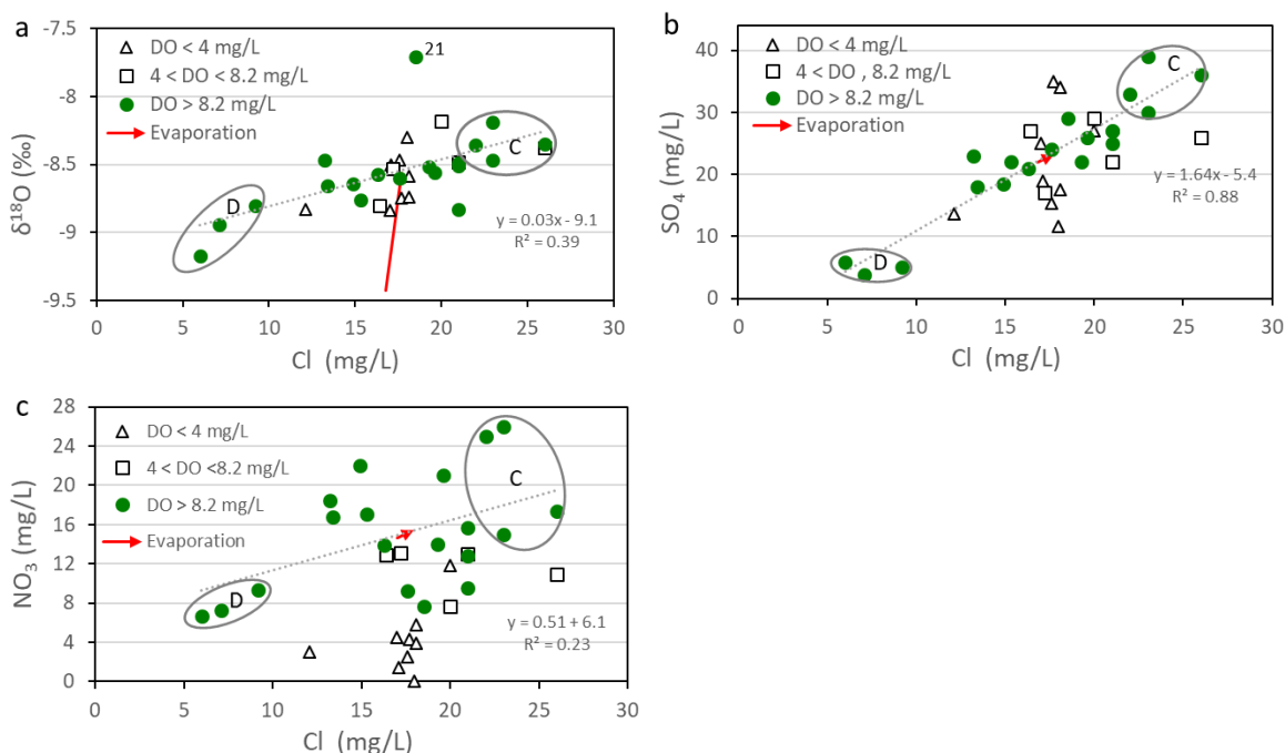
230 Figure 5: Plots of: a. chloride versus water \delta^{18}\text{O} , b. chloride versus sulphate, and c. chloride versus nitrate concentrations. Groups C (with land surface irrigation recharge) and D (alpine river recharge) are circled. The red arrow shows the predicted effect of evaporation.
