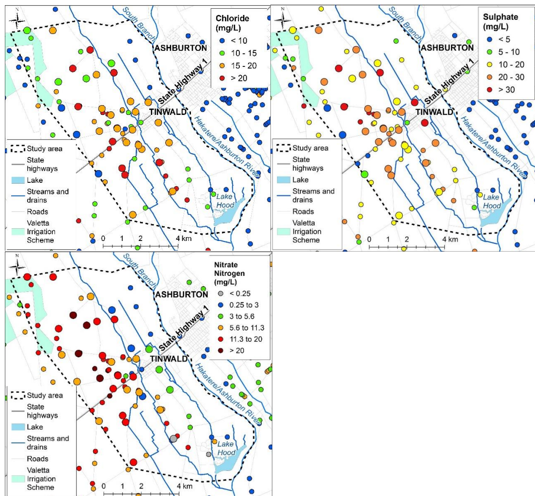
Figure 4: a. Chloride, b. Sulphate, c. Nitrate concentrations in the Tinwald study area (the smaller dots indicate maximum concentrations measured prior to the 2018 investigation). Base maps © LINZ (2019).
