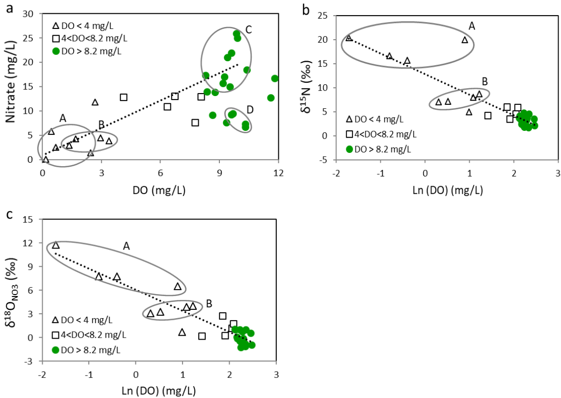
Figure 11: a. Plot of DO versus nitrate concentration. b, c. Plots of \text{Ln}(\text{DO}) versus \delta^{15}\text{N} and \delta^{18}\text{O}_{\text{NO}_3} .
