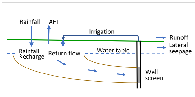
Figure 9: Schematic view of recharge and irrigation return flow in the Tinwald hot spot.
