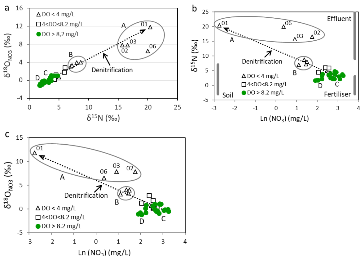
310 Figure 8: a. Plot of \delta^{15}\text{N} versus \delta^{18}\text{O}_{\text{NO}_3} . Groups A and B are circled, C and D indicated by letters. b, c. Plots of \delta^{15}\text{N} and \delta^{18}\text{O}_{\text{NO}_3} versus the natural log of the nitrate concentration.
