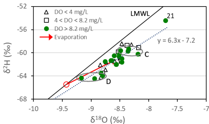
Figure 7: Paired \delta^2\text{H} and \delta^{18}\text{O} data in the Tinwald study area. The average initial composition of the well waters is indicated by the small red circle. Groups C and D samples are circled.
