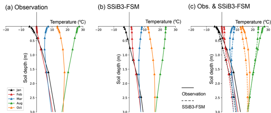
Fig. 5 The seasonal soil temperature profile over NC (16 sites) for 1981–2005. (a) Observation; (b) simulated by SSiB3-FSM; (c) observation and SSiB3-FSM.
