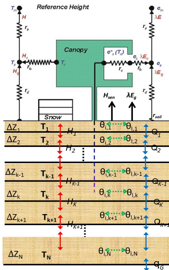
Fig. 1 Schematic diagram of SSiB3-FSM. Soil temperature, soil volumetric water content and soil volumetric ice content are T , \theta and \theta_i , respectively. The heat and water flux between soil layers are represented by H and Q . The soil layer number is k , which ranges from 1 to N .
