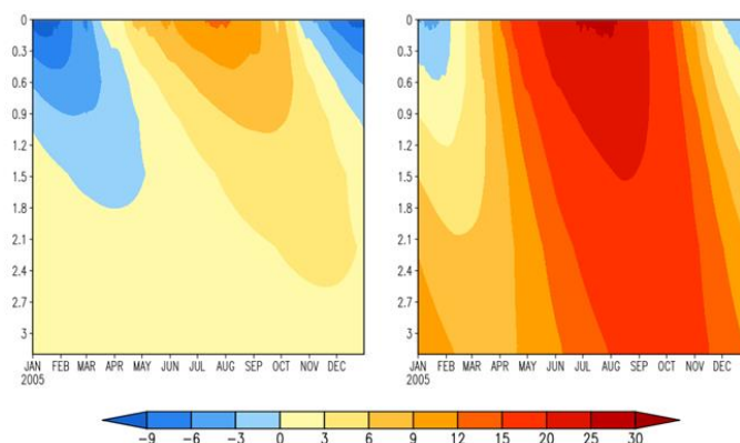
440 Fig. 11 The climatology of simulated daily soil temperature (Left) over the TP (14 sites averaged) and (Right) NC (16 sites averaged) for 1981–2005 (Unit: °C).
