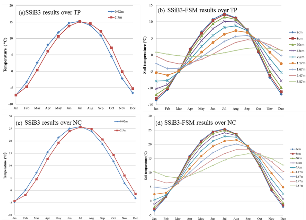
330 Fig. 6 The seasonal soil temperature simulated by SSiB3 and SSiB-FSM over the TP (14 sites) and NC (16 sites) for 1981–2005. (a) The seasonal climatology of T_{gs} (0.02 m) and T_d (2.5 m) by SSiB3 over the TP; (b) the seasonal temperature climatology by SSiB3-FSM over the TP; (c) the seasonal climatology of T_{gs} (0.02 m) and T_d (2.5 m) by SSiB3 over NC, and (d) the seasonal temperature climatology by SSiB3-FSM over NC.
