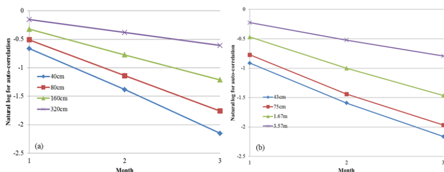
Fig. 9 The natural log for the auto-correlation of over NC for 1981–2005. (a) Observed; (b) SSiB3-FSM.
