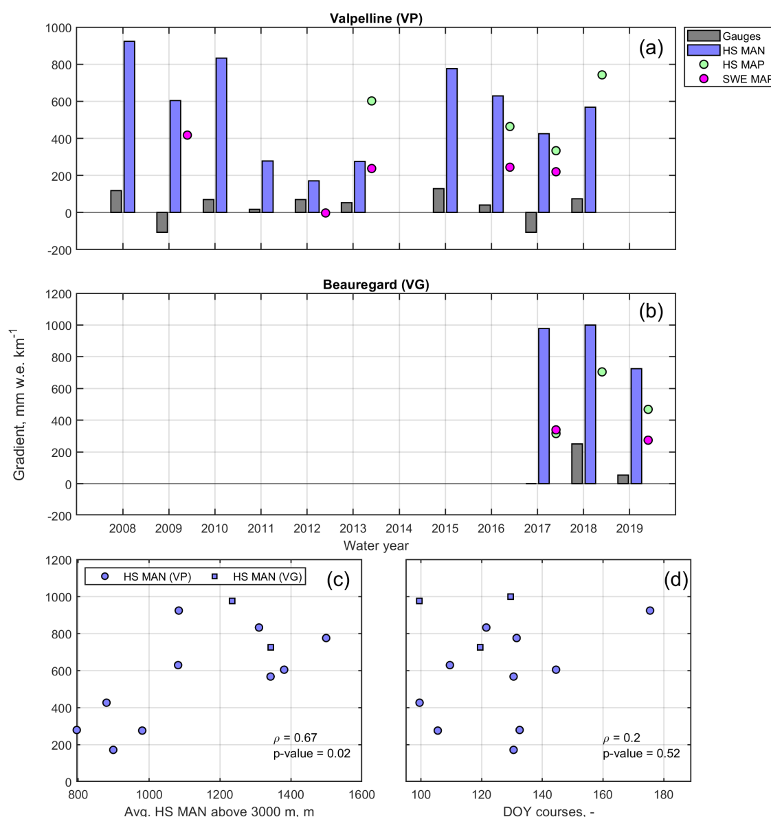
Figure 5. Annual winter orographic gradients estimated by precipitation gauges, snow courses (HS MAN), and the two snow maps assimilated by Flood-PROOFS at Valpelline (a) and Beauregard (b). HS map and SWE map are the snow-depth-sensor map and the SWE map, respectively. Details on Flood-PROOFS and these assimilated maps are reported in Section 3.3. Panels (c) and (d) show estimated orographic gradients by snow courses as a function of mean course snow depth above 3000 m ASL (Avg. HS MAN) and survey day of the year (DOY), respectively. \rho is Pearson's correlation coefficient.
