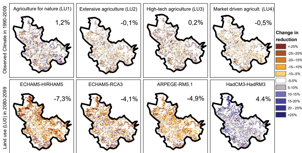
395 Figure 3: Difference in nitrate reduction potential maps between: Top row - Four land use scenarios LU1-4 (Scenario 2-5) and the baseline scenario with land use 0 (Scenario 1). Bottom row: The four future climate model scenarios (scenarios 26, 31, 36, 41) and the reduction maps for the corresponding climate model reference period (scenarios 6, 11, 16, 21) all for land use 0.
