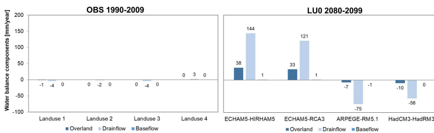
Figure 45: The change in the distribution of the water balance components in mm/year caused by changes in land use and climate change. Left – The difference for the four land use scenarios LU1-4 (Scenario 2-5) and the baseline scenario with land use 0 (scenario 1). Right: The difference between the four future climate model scenarios (scenarios 26, 31, 36, 41) and the corresponding climate model reference period (scenarios 6, 11, 16, 21) all for land use 0 (modified from Karlsson et al. (2016)).
