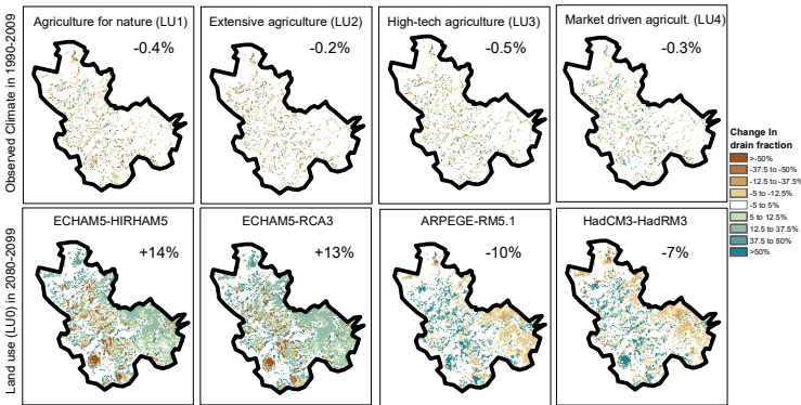
540 Figure 56: Changes in the drain flow fraction from baseline (LU0) to the four land use scenarios (LU1-4) in the observational period (top row) and from the reference period to the future period for four climate models using LU0 (bottom row). Drain flow fraction is defined as drain flow divided by net precipitation. Green colors indicate that a larger percentage of the net precipitation is channeled into the drains for the future. Number in upper right corner indicate the relative change in drain flow fraction from reference period to future period. The corresponding percentage of drain flow in the baseline scenario is 31%.
