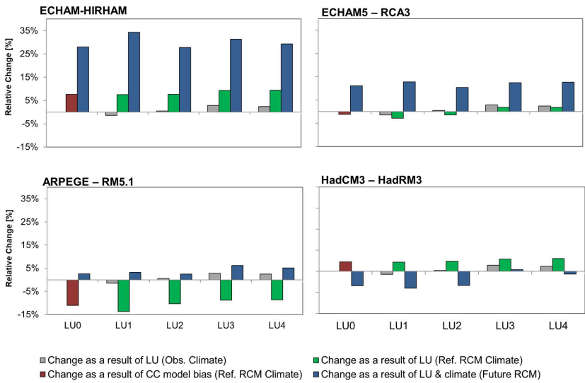
Figure 69: Bars denote the change in nitrate flux at the catchment outlet that arises from using either a fixed the-baseline-nitrate 640 reduction potential map (baseline) or using a the reduction map based on the individualfrom-the scenarios. The scenarios encompass cases with different land use (grey), climate model data for the present (red bar) with land use changes (green bars) or future climate data and land use changes (blue bars).
