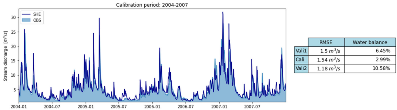
Figure S1: Left - Hydrograph of the main discharge station for observed and simulated flow at the outlet (Kratholm) during the calibration period. Right – Table of performance during the calibration (2004-2007), the validation period 1 (2000-2003) and validation period 2 (2008-2009). Figure modified from Karlsson et al. (2016).
