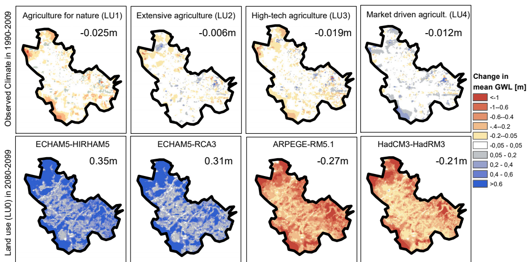
Figure S4: Changes in groundwater level from the upper saturated layer. Changes are reported as change from (LU0) to LU1-4 with observational climate for the top row and from RCM reference period to RCM future period for the bottom row. Figure modified from Karlsson et al. (2016).
