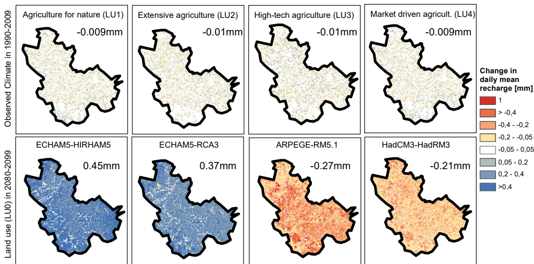
Figure S3: Changes in daily recharge from baseline (LU0) to the four land use scenarios (LU1-4) in the observational period (top row) and the change for four climate scenarios (LU0) from reference to future period (bottom row).
