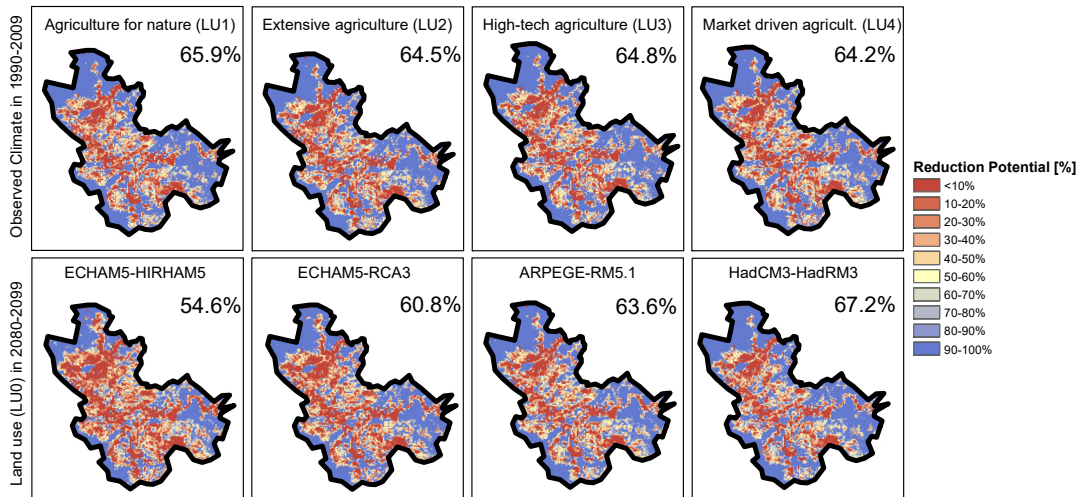
Figure S2: Nitrate reduction potential maps for four land use scenarios (LU1-4) in the observational period (top row) and four climate scenarios (LU0) for the future climate (bottom row), showing the fraction of the added nitrate that is reduced for each grid. In the top row observed climate is used, changing only the land use (scenarios 2-5). In the bottom row the present land use (LU0) is used, while using future climate projected by the four climate models (scenarios 26, 31, 36 and 41).
