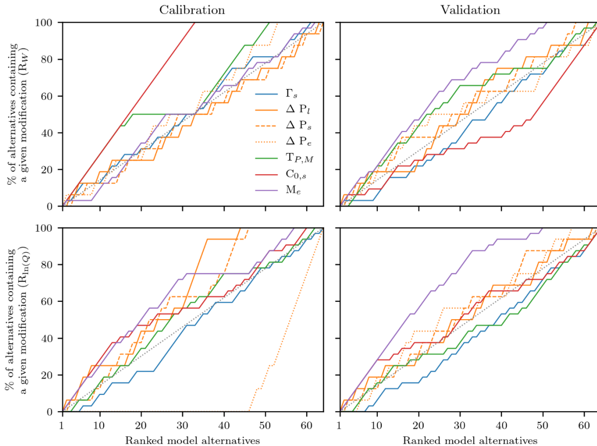
475 Figure 8 Cumulative plots for each of the 7 individual modifications to the snow routine of the HBV model as a function of the ranked 64 model structures arising from all the possible combinations of modifications. The modifications are a seasonally-variable temperature lapse rate ( \Gamma_s ), a linear, sinusoidal, and exponential function for the precipitation phase partition ( AP_l , AP_s , and AP_e respectively), different thresholds for precipitation phase and snowmelt ( T_{P,M} ), a seasonally variable degree-day factor ( C_{0,s} ), and an exponential snowmelt with no refreezing ( M_e ). Model simulations against snow water equivalent are presented in the top row, while those against logarithmic stream runoff are presented in the bottom row. Model calibration is presented in the left column and model validation in the right one. Model modifications plotting above the 1:1 line (grey dotted line) tend to be included in high-ranking model structures, while those plotting below the 1:1 line tend to be included in low ranking structures.
