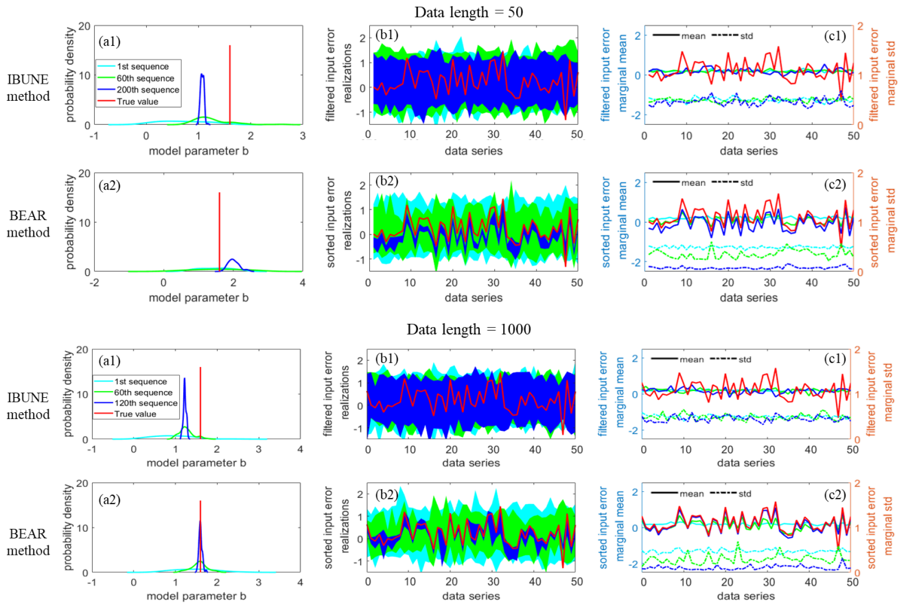
460 Figure 5 Comparison of the results for scenario 1 in the synthetic case 1, the ensemble particle size of N=100 at different sequences of calibration (represented in different colours), via different methods (row 1: IBUNE method; row 2: BEAR method) and under different data lengths in calibration (the upper group: data length is 50; the lower group: data length is 1000, selects 50 data the same as the upper group to show). Column a shows the probability density of model parameter b at different sequences of calibration. The other model parameters have the same pattern of change and thus there is no need to show. Column b shows the value interval of input error realizations of 100 particles after reordering in the BEAR method or filtering in the IBUNE method and Column c shows the corresponding marginal mean and standard deviations at each time step. The 1 st sequence (in cyan) shows the raw input 465 errors of random sampling, before reordering or filtering.
