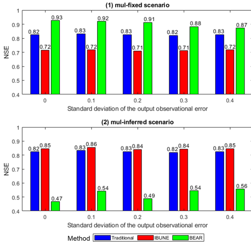
450 Figure 3 Comparison of Nash-Sutcliffe efficiency (NSE) of the modified input v.s true input under the interference of the output observational errors with the increasing standard deviations in two calibration scenarios in the synthetic case 2 (including mul-fixed and mul-inferred ; notations are given in Table 2) via three calibration methods (including the Traditional method, the IBUNE method and the BEAR method, their algorithms are explained in Sect. 2.4)
