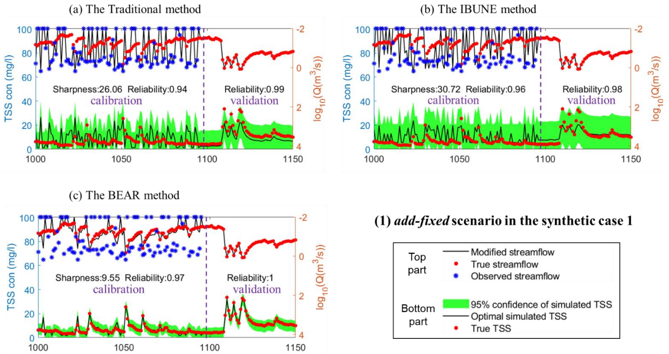
515 Figure B 1(1) Comparison of time series of synthetic data and uncertainty bands estimated via three calibration methods (including the Traditional method, the IBUNE method and the BEAR method; algorithms are explained in Sect. 2.4) for a select period of add-fixed scenarios in the synthetic case 1(notations are given in Table 2)
