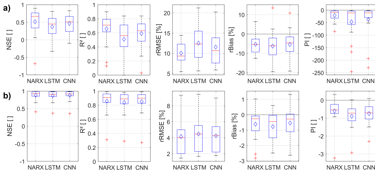
Figure 2. Boxplots showing the seq2val forecast accuracy of NARX, LSTM and CNN models within the test period (2012-2016) for all considered 17 hydrographs. The diamond indicates the arithmetic mean; a) only meteorological inputs; b) GWL_{t-1} as additional Input
