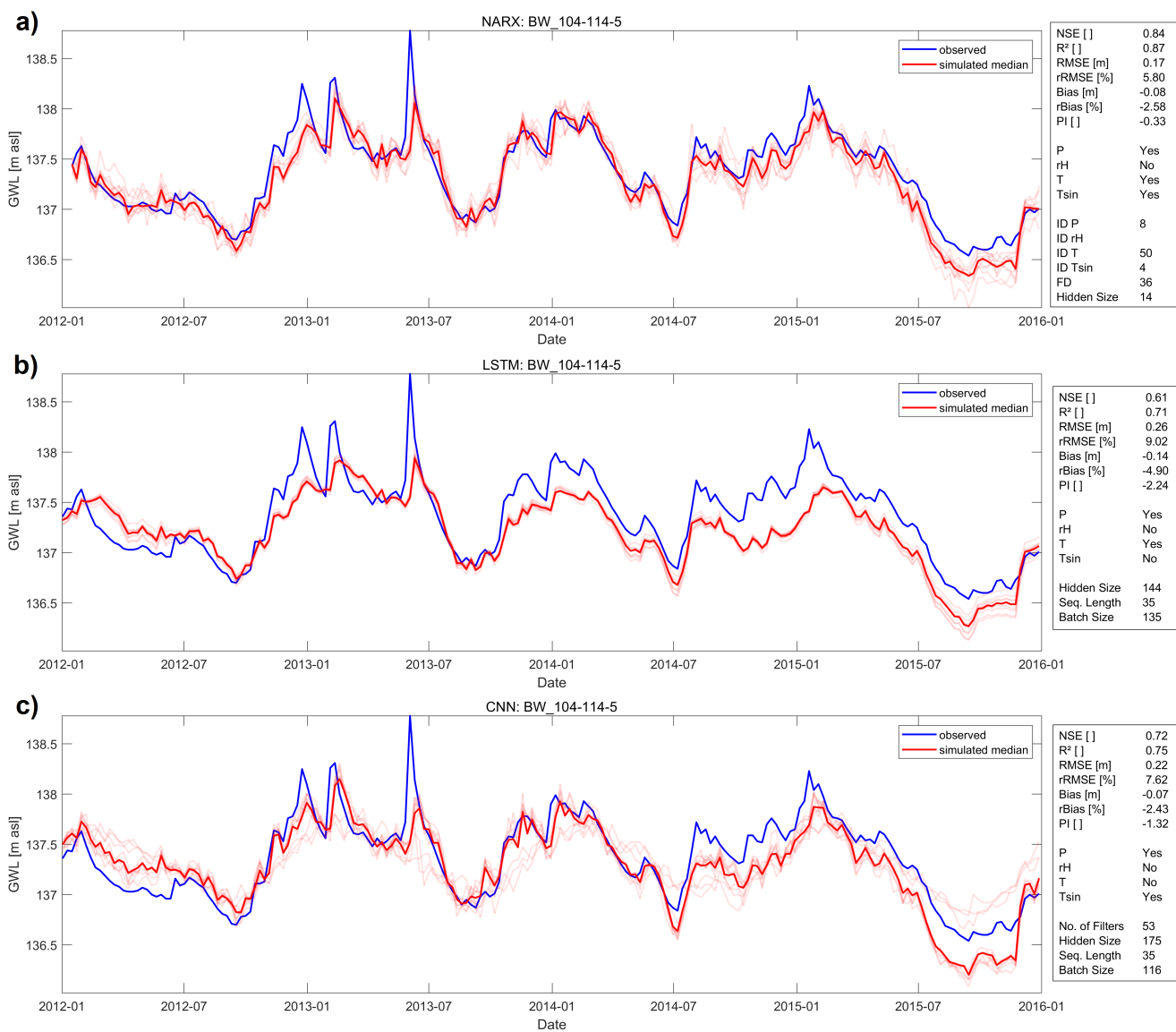
Figure 3. Forecasts of (a) a NARX, (b) a LSTM and (c) a CNN model for well BW_104-114-5 during the test period 2012-2016.
