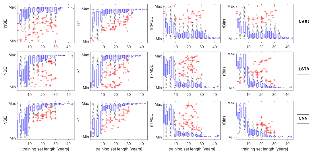
Figure 8. Influence of training data length on model performance.
