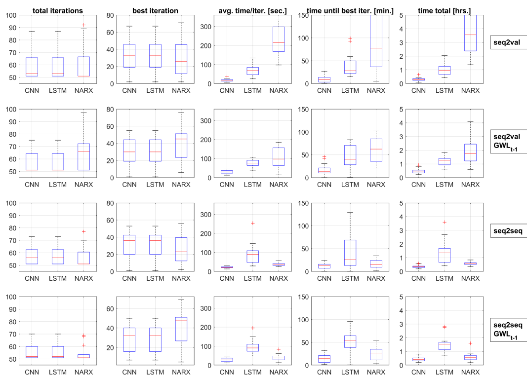
Figure 7. Comparison of the performed HP-optimizations (columns 1 and 2), their calculation time per iteration in seconds (col 3), until the optimum was found (minutes) (col. 4) and the total time spent on optimization in hours (col. 5).
