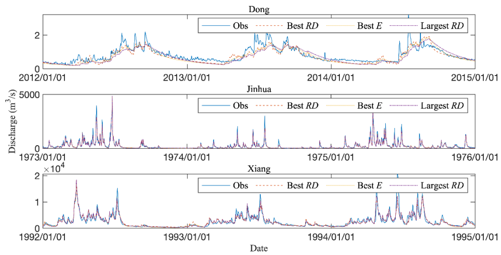
695 Figure 5: Typical examples with best RD , best E and largest RD (representative three-year hydrograph).
