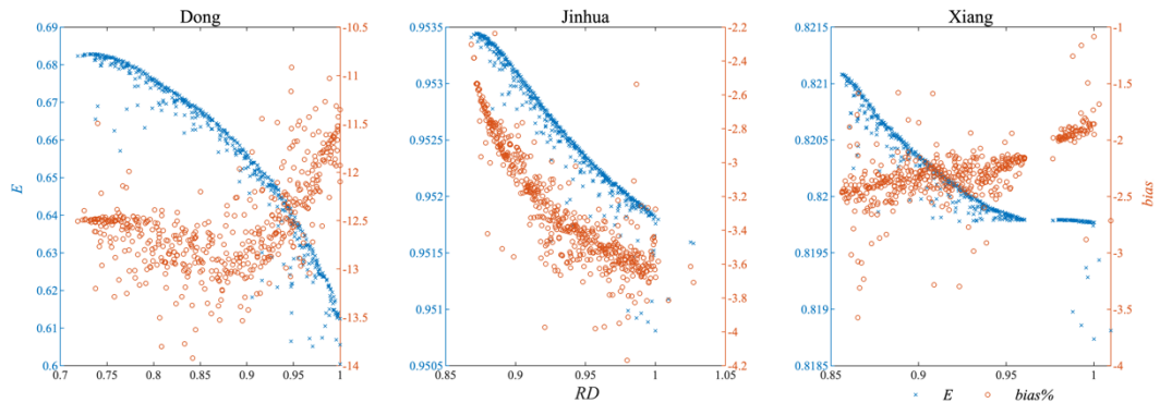
690 Figure 4: E - RD of last generation of GA calibration.
