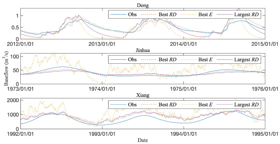
Figure 15: Baseflow of typical models and observations (representative three-years hydrograph).
