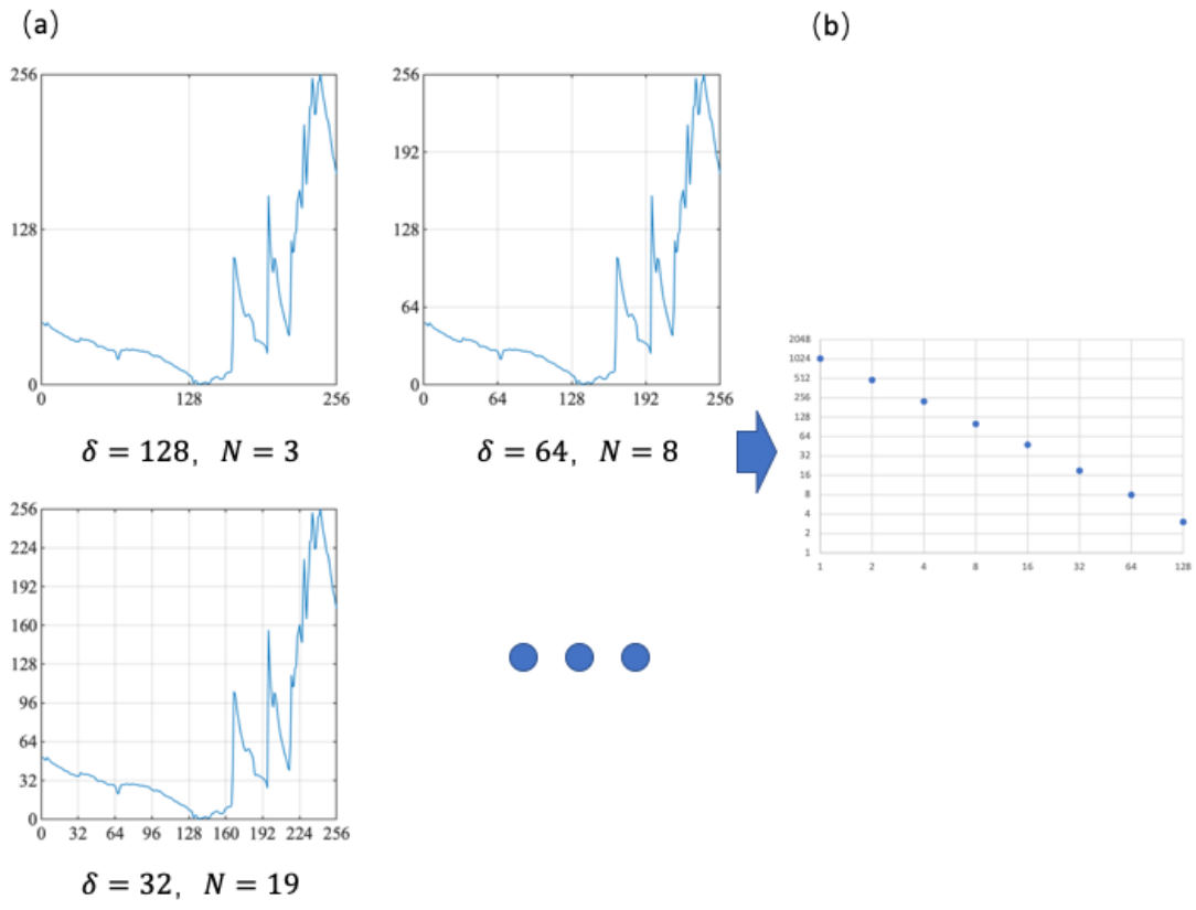
Figure 1: Flow chart of using box-counting method to calculate the Hausdorff dimension of time series.
