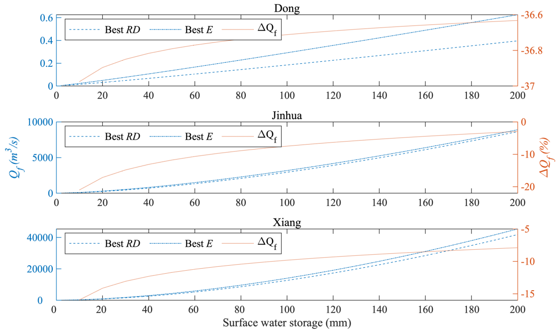
Figure 9: Response of fast flow to surface water storage. For each case, fast flow responses of typical models with best RD and E are presented.
