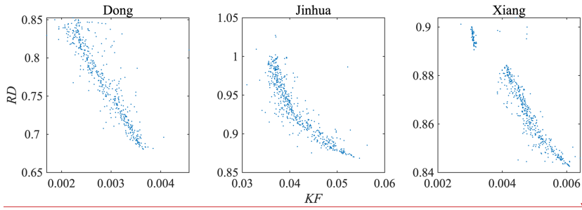
Figure 8: KF and RD relationship in three cases.
