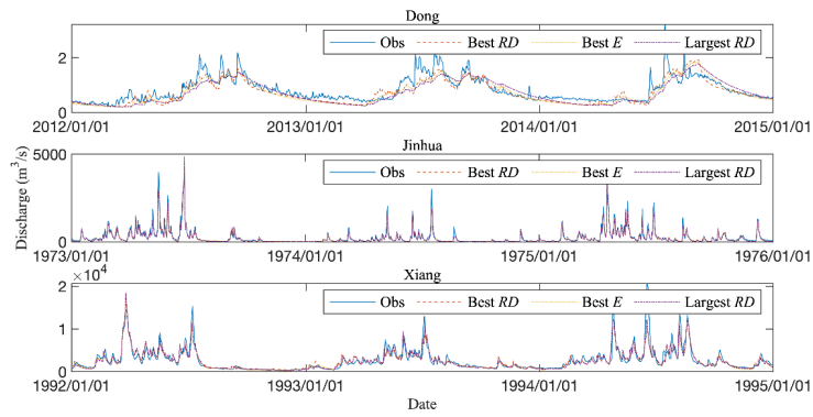
Figure 5: Typical examples with best RD , best E and largest RD (representative three-year hydrograph).
