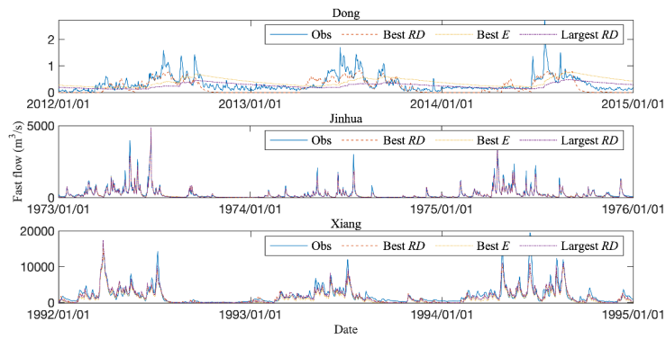
Figure 14: Fast flow of typical models and observations (representative three-years hydrograph).
