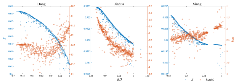
Figure 4: E - RD of last generation of GA calibration.
