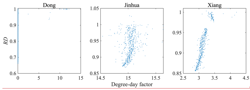
Figure 12: Degree-day factor and RD relationship in three cases.
