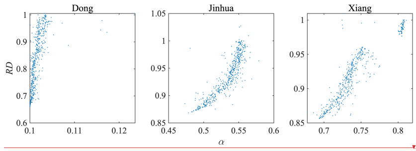
Figure 7: \alpha and RD relationship in three cases.
