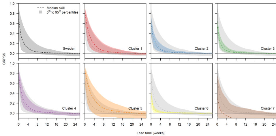
Figure 8 Streamflow forecast skill (in terms of CRPSS) as a function of lead time for the entire country (top-left corner; also shown in Figure 3a) and each of the 7 clusters. The median skill and range for Sweden are provided in the background of clusters 1-7 to provide a reference for the values of each cluster.
