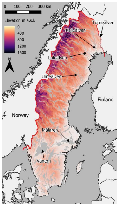
500 Figure A1 Map of Sweden showing its topography and main hydrographic network. The rivers and lakes referred to in the main text are indicated here for convenience.
