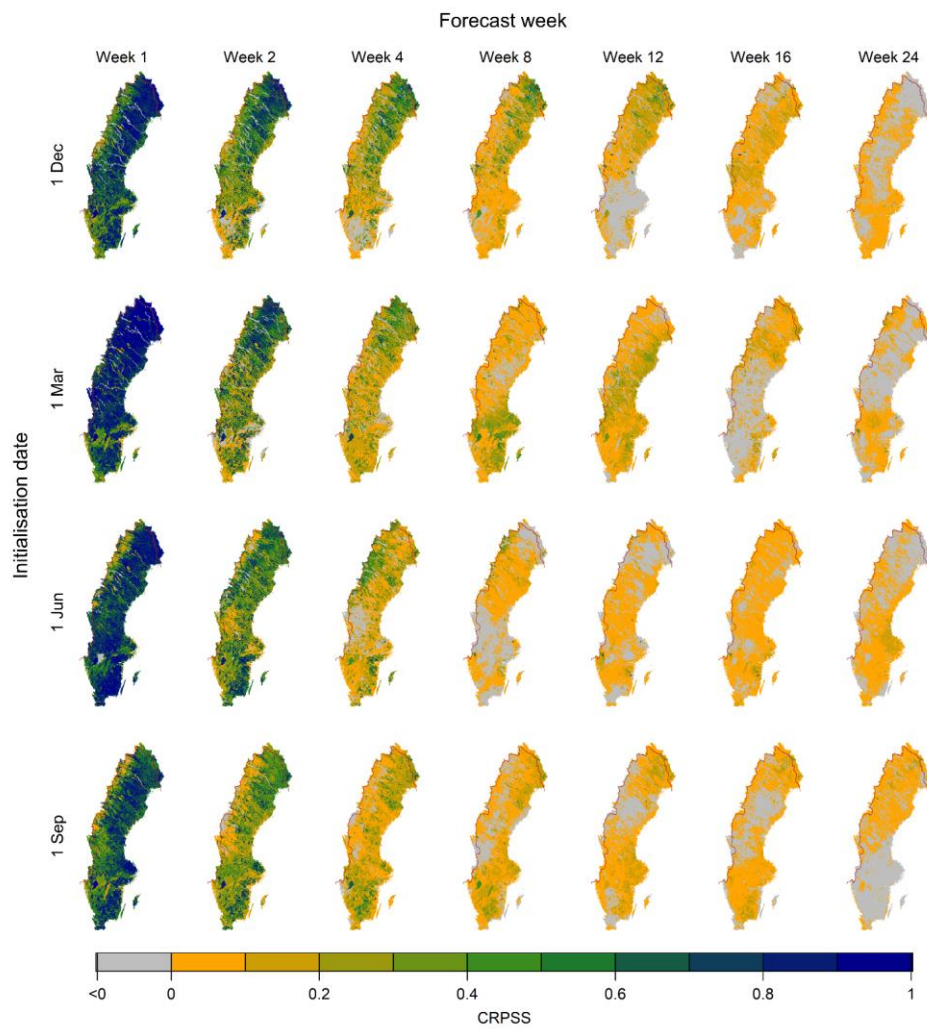
245 Figure 4 Spatial distribution of streamflow forecast skill (in terms of CRPSS) for selected initialisation dates (rows) and forecast time horizons (columns).
