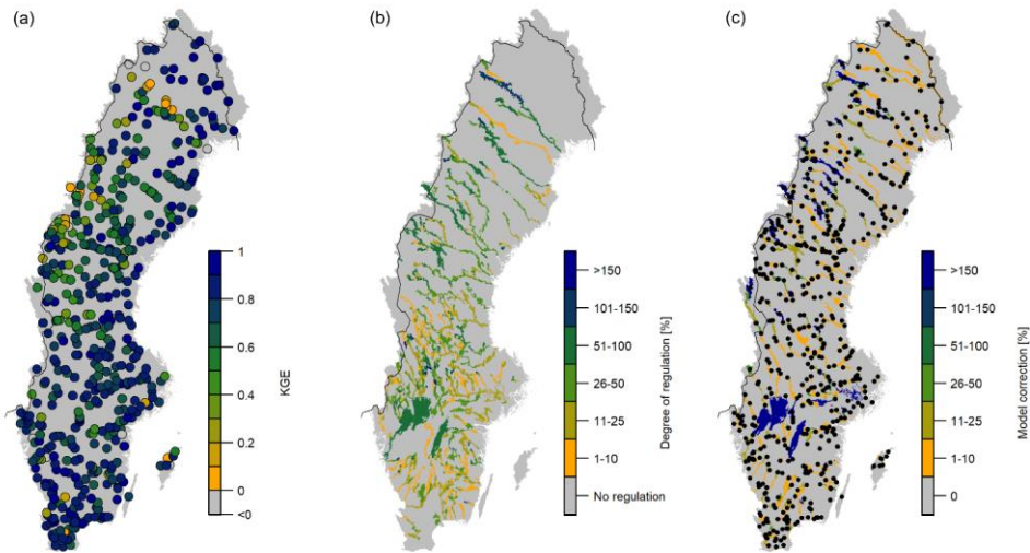
Figure 1 Study domain: (a) S-HYPE model Kling-Gupta efficiency (KGE) for the period 1981 – 2016 for each of the 539 hydrological stations, (b) degree of regulation of each S-HYPE catchment, and (c) average model correction value for each S-HYPE catchment following the autoregressive correction method.
