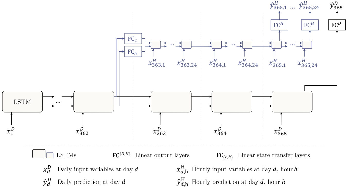
Figure 2. Illustration of the multi-timescale LSTM architecture that uses one distinct LSTM per timescale. In the depicted example, the daily and hourly input sequence lengths are T^D = 365 and T^H = 72 . In the sMTS-LSTM model (i.e., without distinct LSTM branches), FC_c and FC_h are identity operations, and the two branches (including the fully-connected output layers FC^H and FC^D ) share their model weights.
