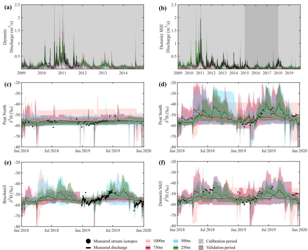
780 Figure 3: Simulated discharge at (a) Demnitz, and (b) Demnitz Mill, and stream isotopes at (c) Peat North, (d) Peat South, (e) Bruchmill and (f) Demnitz Mill. Colours indicate the model resolution, with solid lines showing the median simulation and shaded regions showing the upper and lower simulation bounds.
