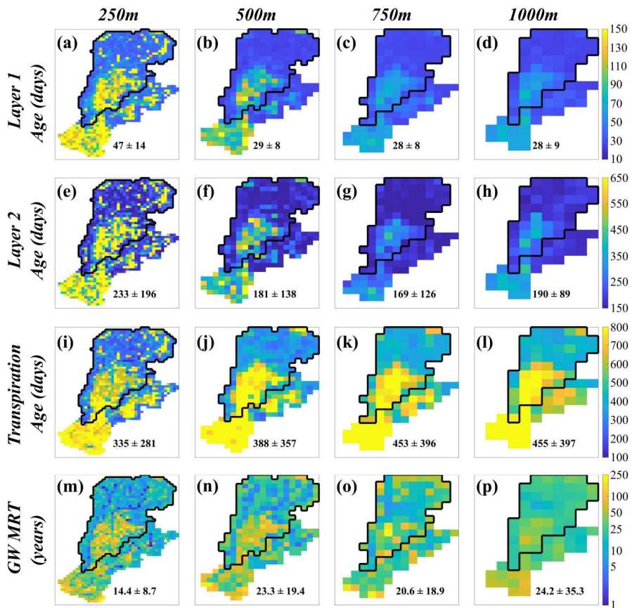
800 Figure 7: Estimated average water ages during the summer (Jun – Aug) in (a-d) soil layer 1, (e-h) layer 2, and (i-l) transpiration, and (m-p) long-term groundwater mean residence time (GW MRT) for model resolutions 250, 500, 750, and 1000m, respectively. Note: groundwater residence times are in years. Black boundaries show the calibration extent of the Demnitz Mill sub-catchment. Values shown are the catchment-wide long-term (2009 – 2019) average values and average standard deviation (average of each pixel) within the Demnitz Mill sub-catchment.
