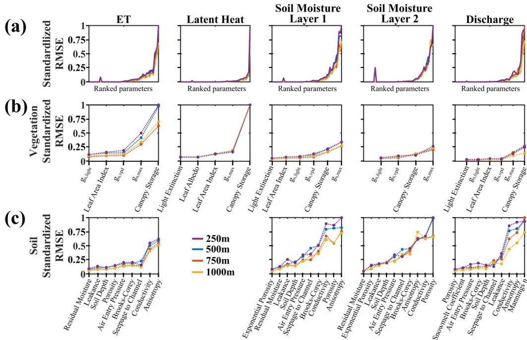
775 Figure 2: (a) Standardised root mean square error, (b) standardized root mean square error for the most sensitive vegetation parameters, and (c) standardized root mean square error for the most sensitive soil parameters for each output and spatial resolution. Vegetation parameters, g_s , are the control of vegetation stomatal conductance, with maximum potential conductance ( g_s,max ), light controlling conductance ( g_s,light ), and vapour pressure deficit controlling conductance ( g_s,vpd ).
