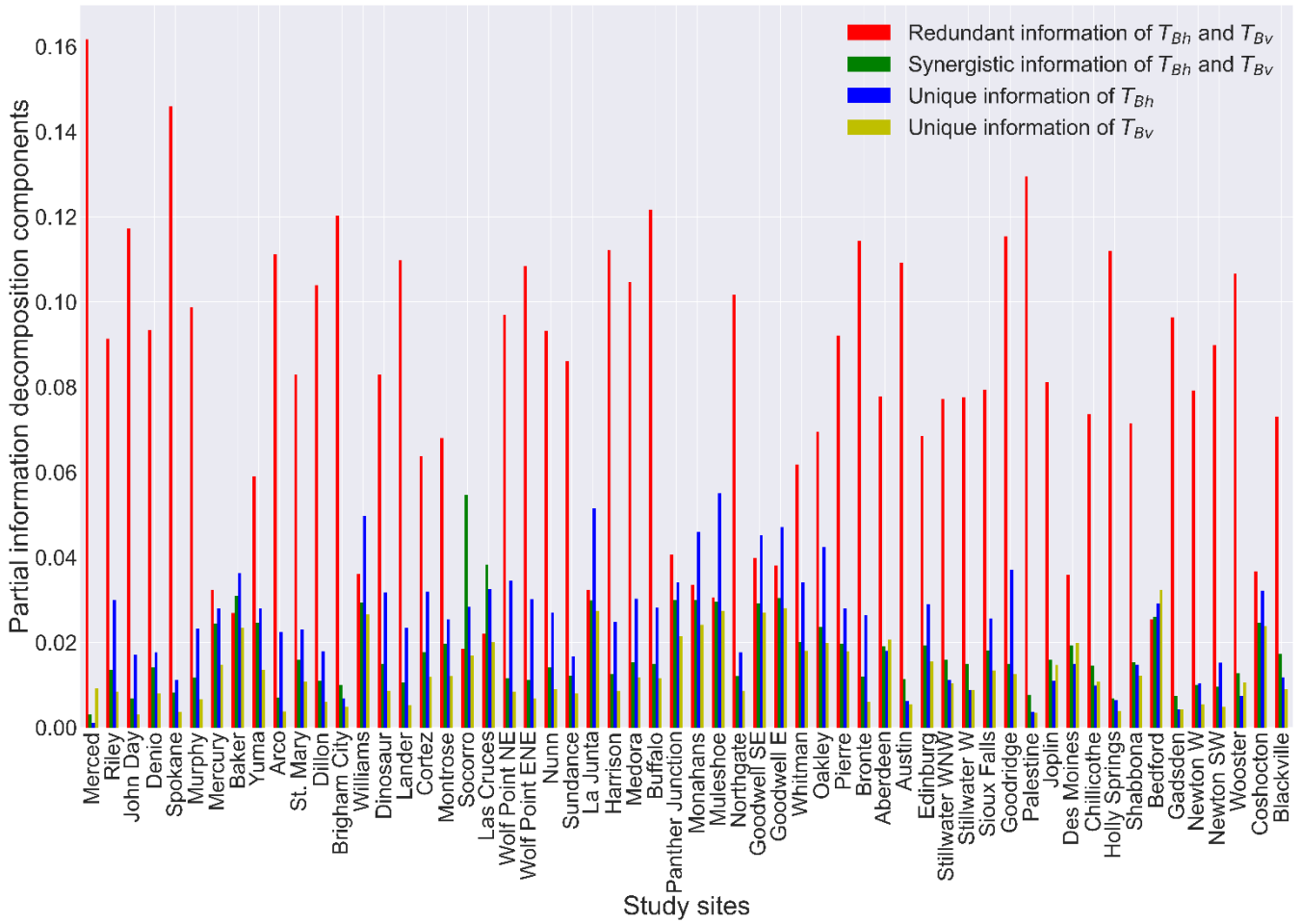
740 Figure 6 Partial information decomposition components between horizontally ( T_{Bh} ) and vertically ( T_{Bv} ) polarized brightness 745 temperature and DCA soil moisture. See figure 2 caption for site ordering.
