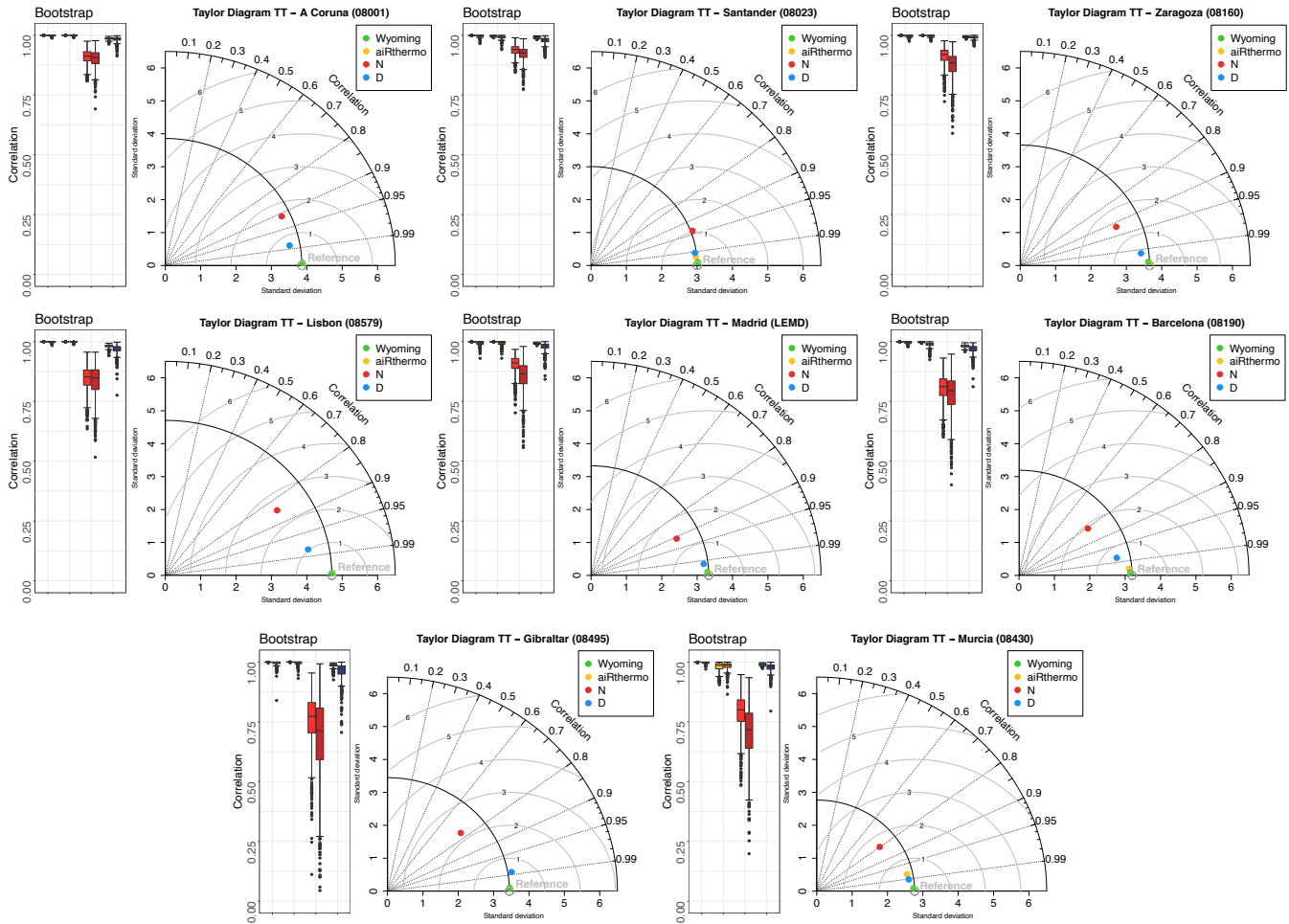
Figure 2. Taylor diagrams showing the r , RMSE and SD values for Wyoming, aiRthermo, N and D compared to TT values computed from IGRA (Reference). On the left side of each Taylor diagram, a Box-Whiskers plot is added in order to show Pearson's and Spearman's correlations between each experiment and the reference data (lighter and darker colours, or first and second columns of the Box-Whiskers respectively). The bootstrap technique with resampling was used to create 1000 synthetic time-series. Wyoming, aiRthermo, N and D are plotted in green, orange, red and blue respectively.
