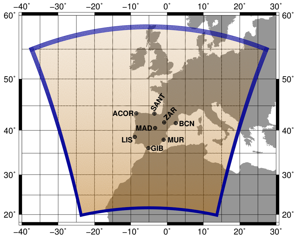
Figure 1. The domain used in both WRF simulations is presented with darkorange dark orange dots, while the darkblue dark blue region highlights the relaxation zone. The location of all the radiosondes available over the IP is also presented with quartered circles.
