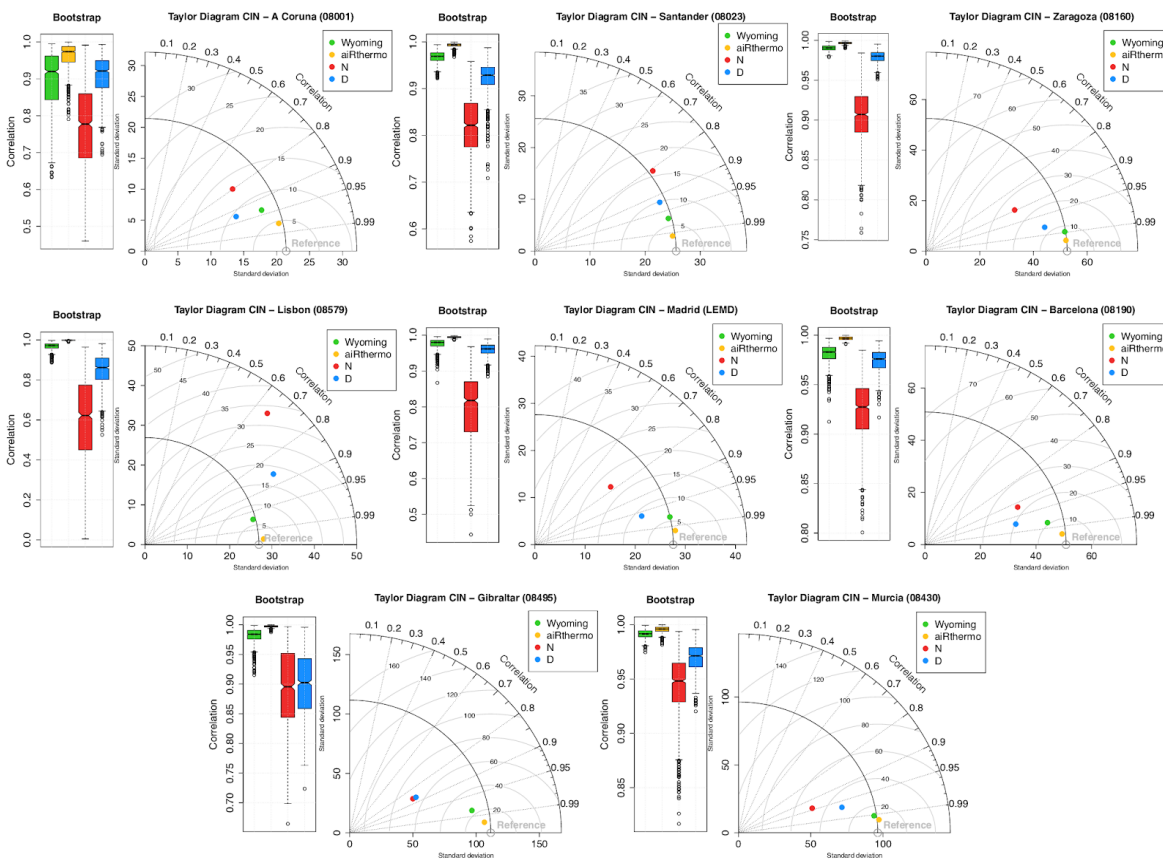
Fig.3. Taylor diagrams of CIN if the values from IGRA are taken as reference.
