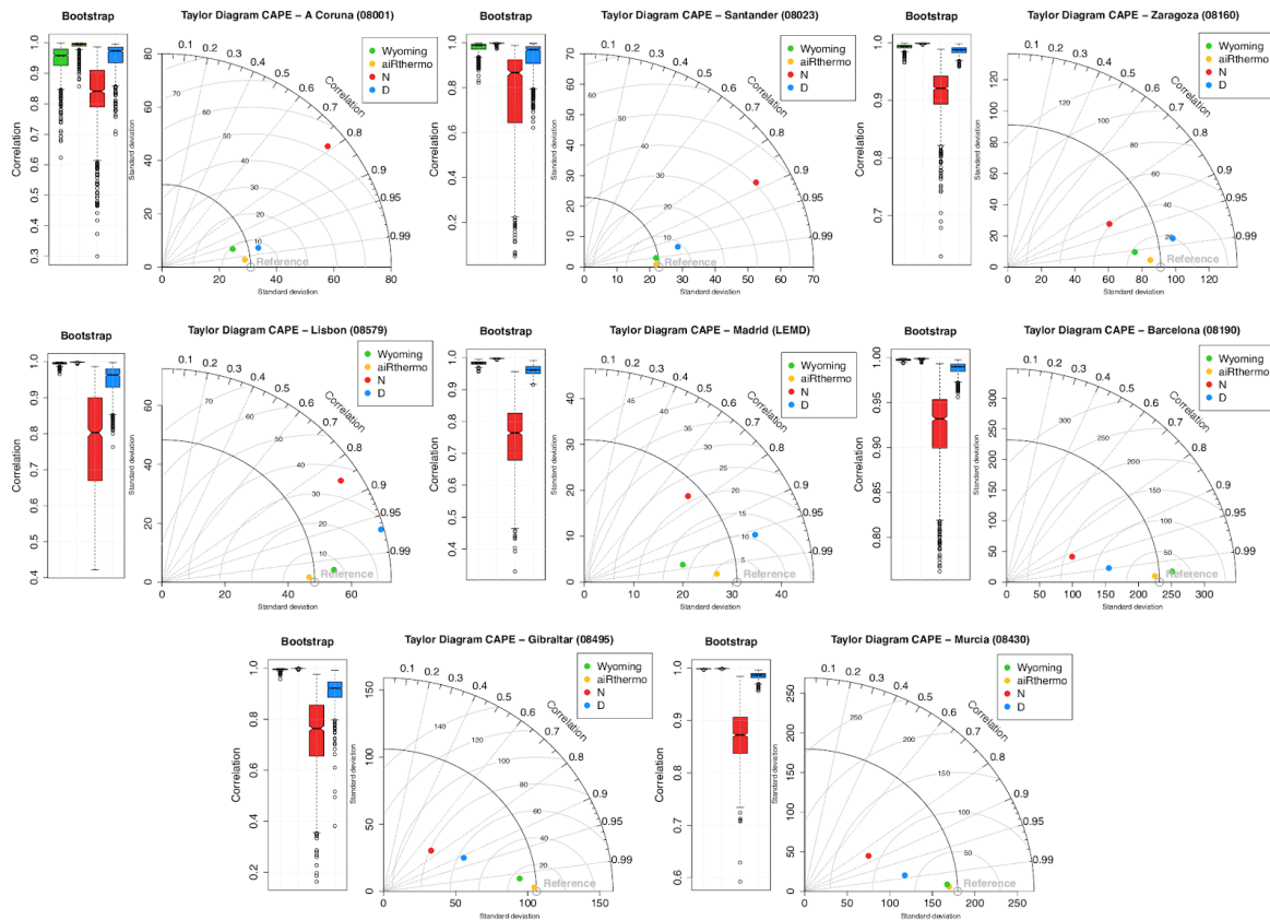
Fig. 2. Taylor diagrams of CAPE if the values from IGRA are taken as reference.
