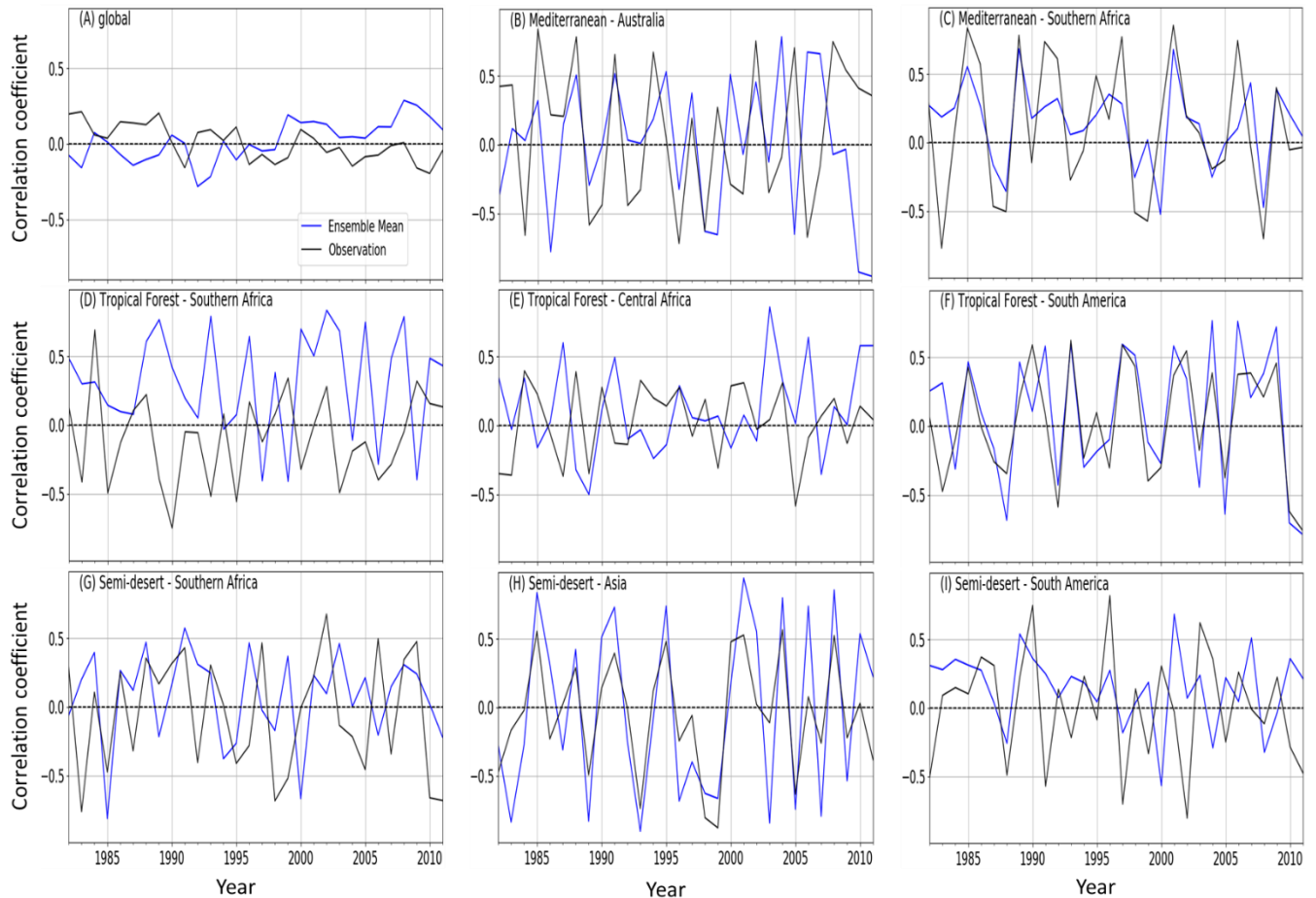
670 Figure 11. Correlations between SPEI (12-month timescale) and ensemble mean of LAI from TRENDY (blue line), GIMMS LAI (black line) for (A) Global (B) Mediterranean vegetation over Australia (C) Mediterranean vegetation over southern Africa (D) Tropical Forest over southern Africa (E) Tropical Forest over Central Africa (F) Tropical Forest over South America (G) Semi-desert biome over southern Africa (H) Semi-desert over Asia and (I) Semi-desert over South America.
