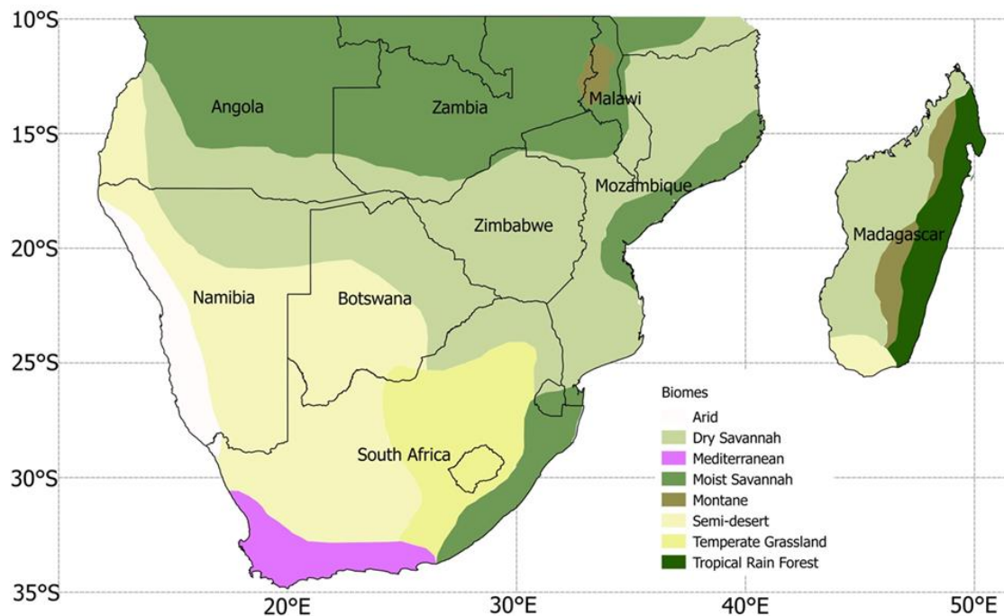
Figure 1. Major vegetation biomes in southern Africa (adapted from UNEP, 2008, Sinclair & Beyers, 2015 and Lawal et al. , 2019a,b). The black lines indicate political boundaries.
