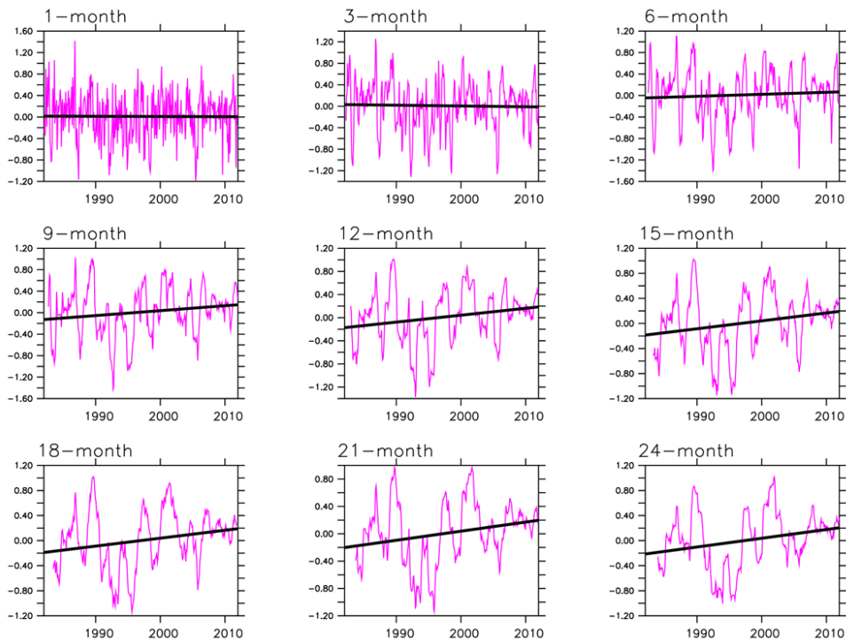
480 Figure 6. Evolution of SPEI in southern Africa for the period 1982 – 2011. The trend is significant at 90% confidence interval for all timescales.
