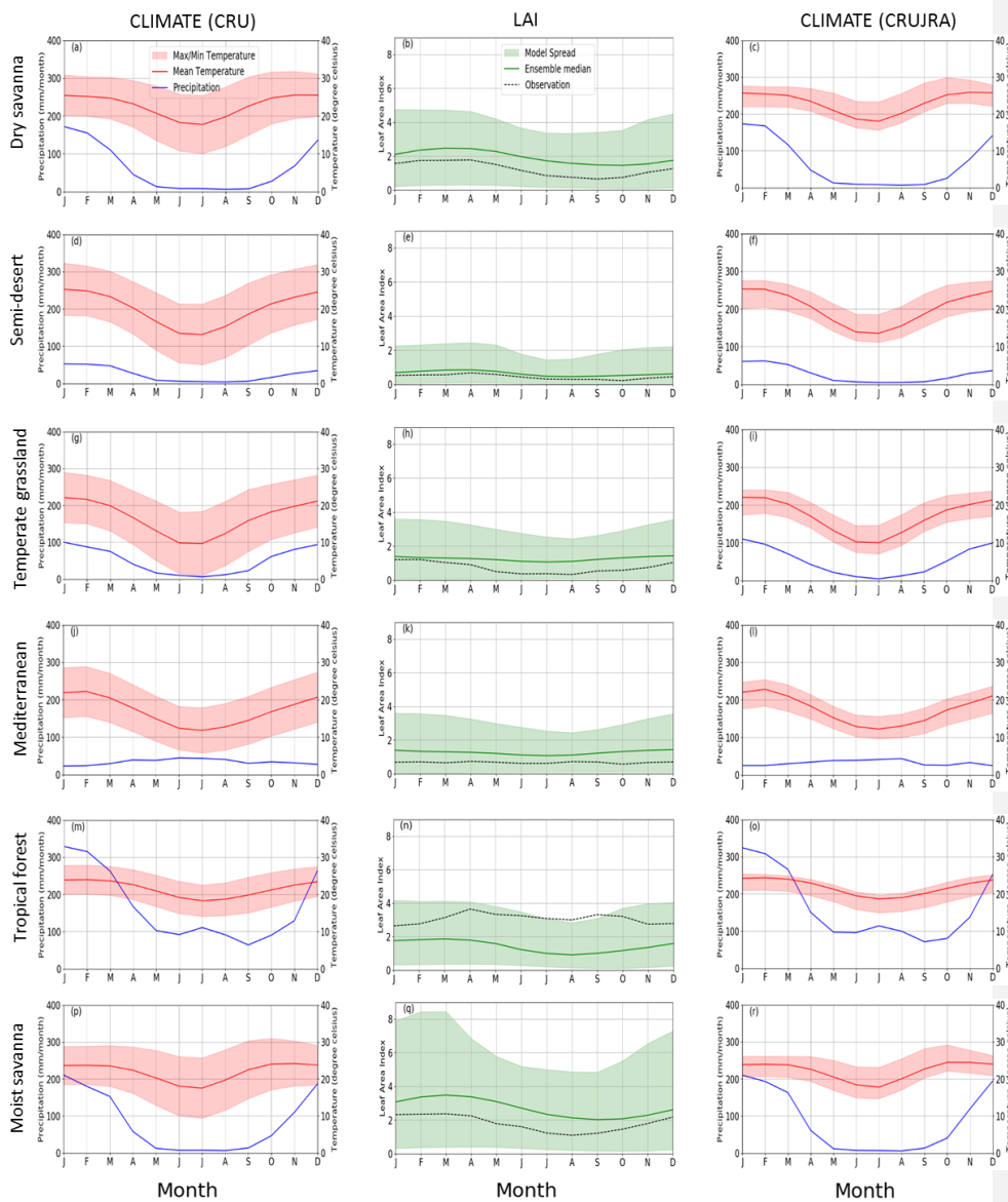
Figure 4. Annual cycle of observed climate variables (precipitation, mm/month; maximum, minimum and mean temperature, °C) and LAI for observation and multi-model mean (TRENDY) across six southern African biomes over for the period 1982 – 2011. The annual cycle of the LAI for individual models are shown in Figure S5.
