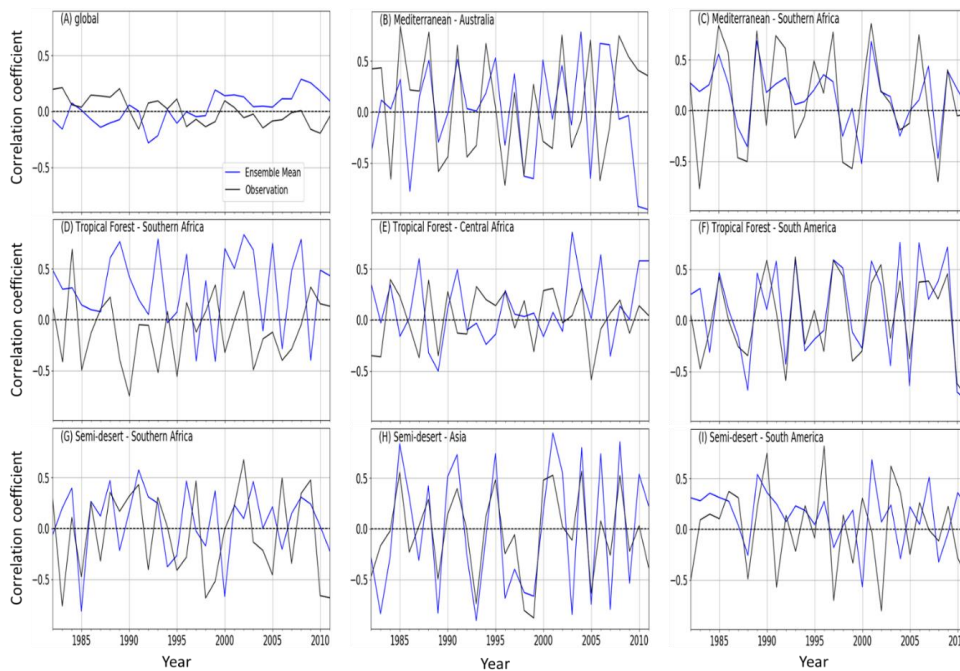
715 Figure 11. Correlations between SPEI (12-month timescale) and ensemble mean of LAI from TRENDY (blue line), GIMMS LAI (black line) for (A) Global (B) Mediterranean vegetation over
