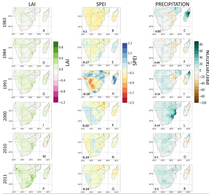
680 Figure 10. Spatial pattern changes in satellite-calculated LAI, observed SPEI and precipitation during extreme dry (1983, 1984, 1991) and wet (2000, 2010, 2011) years. For (A) – (I), the changes in LAI, SPEI and precipitation were calculated as a difference between the dry year and the 30-year mean, and for (J) – (R), changes in LAI, SPEI and precipitation 685 were calculated as the difference between the wet year and the 30-year mean. White areas indicate no correlation. The inset numbers in the second column are the pattern correlation coefficient values between the LAI and SPEI for the extreme dry and wet years, while the values in the third column are the pattern correlation coefficient values between LAI and precipitation during the extreme dry and wet years.
