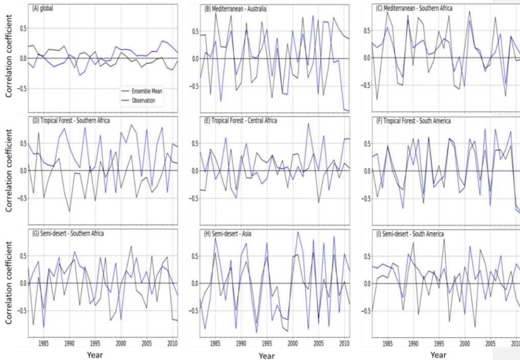
670 Figure 11. Correlations between SPEI (12-month timescale) and ensemble mean of LAI from TRENDY (blue line), GIMMS LAI (black line) for (A) Global (B) Mediterranean vegetation over Australia (C) Mediterranean vegetation over southern Africa (D) Tropical Forest over southern Africa (E) Tropical Forest over Central Africa (F) Tropical Forest over South America (G) Semi- desert biome over southern Africa (H) Semi-desert over Asia and (I) Semi-desert over South 675 America.
