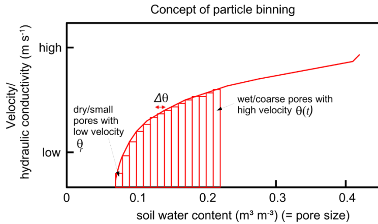
Figure 1. Particle binning concept. All particles within an element of the Euler-Grid are distributed to bins (= red rectangles) representing fractions of the actual soil water content stored in different pore sizes. Displacements of these particle fractions are determined by the corresponding flow velocities and diffusivities (figure taken from Sternagel et al. (2019)).
