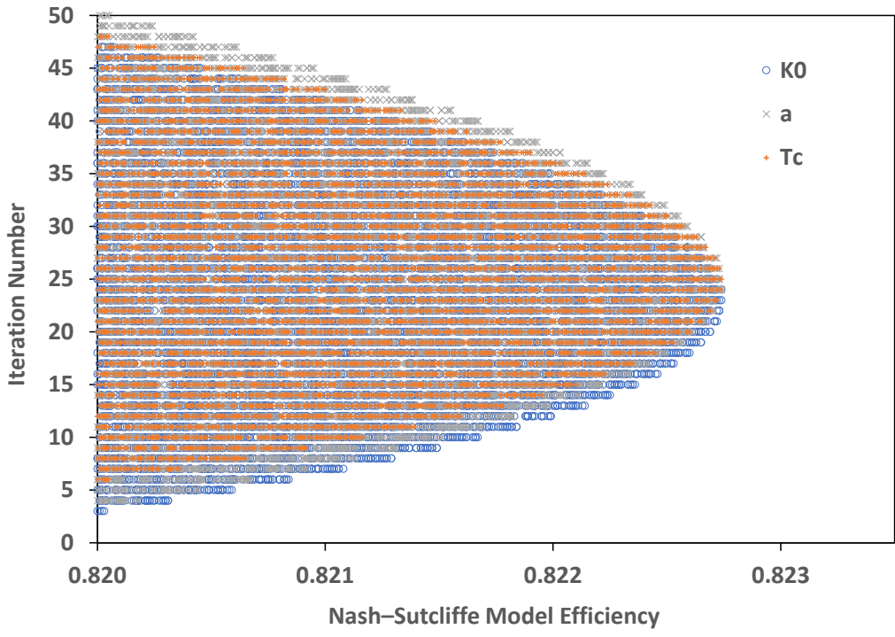
Figure RC1-1: Solutions for k_0 , T_c , and a using NSE as the criteria. Ranges of parameter values: 0.006 < k_0 < 0.009 , 430 < T_c < 770 , 36 < a < 55 .
